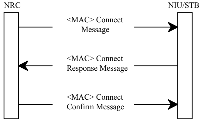
Figure 2-19 Connection Establishment Signaling Sequence
