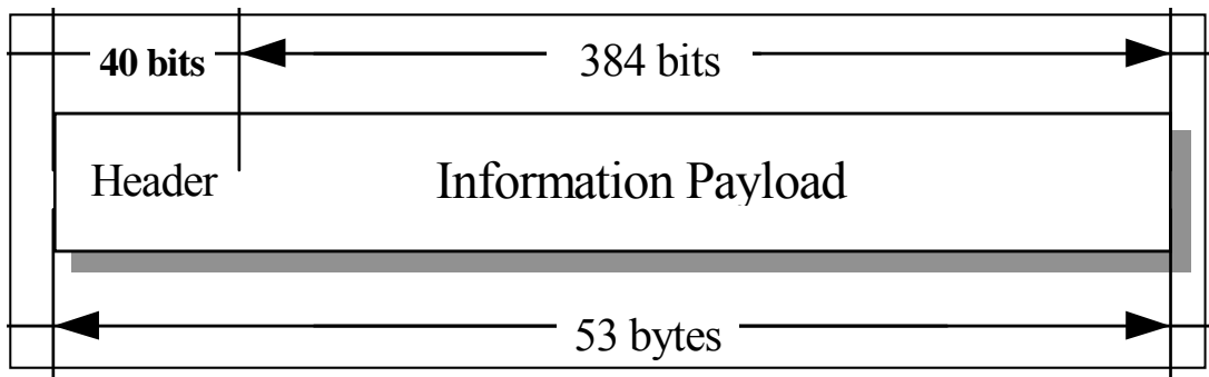
Figure 2-12 ATM Cell Structure
