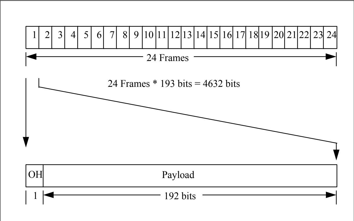
Figure 2-5 SL-ESF Frame Structure
