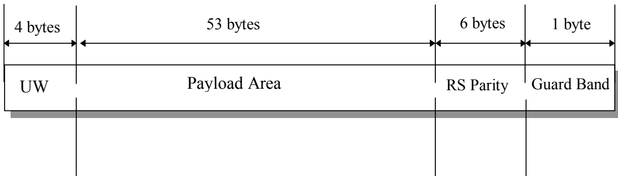
Figure 2-14 Upstream Slot Structure
