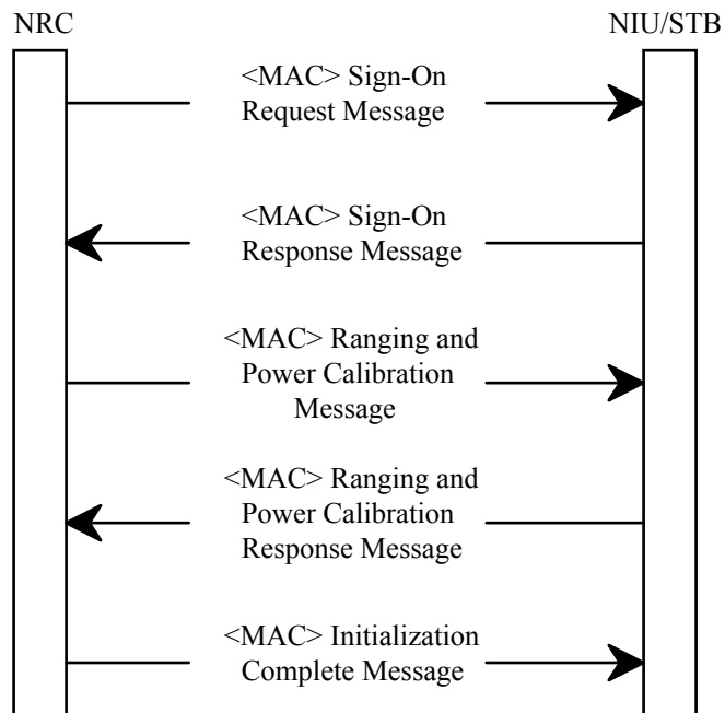
Figure 2-17 Sign-On Messaging Sequence
