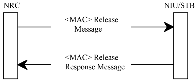
Figure 2-20 Connection Release Signaling
