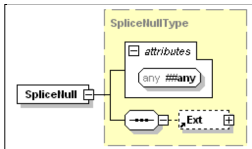
Figure 8-2. SpliceNull
