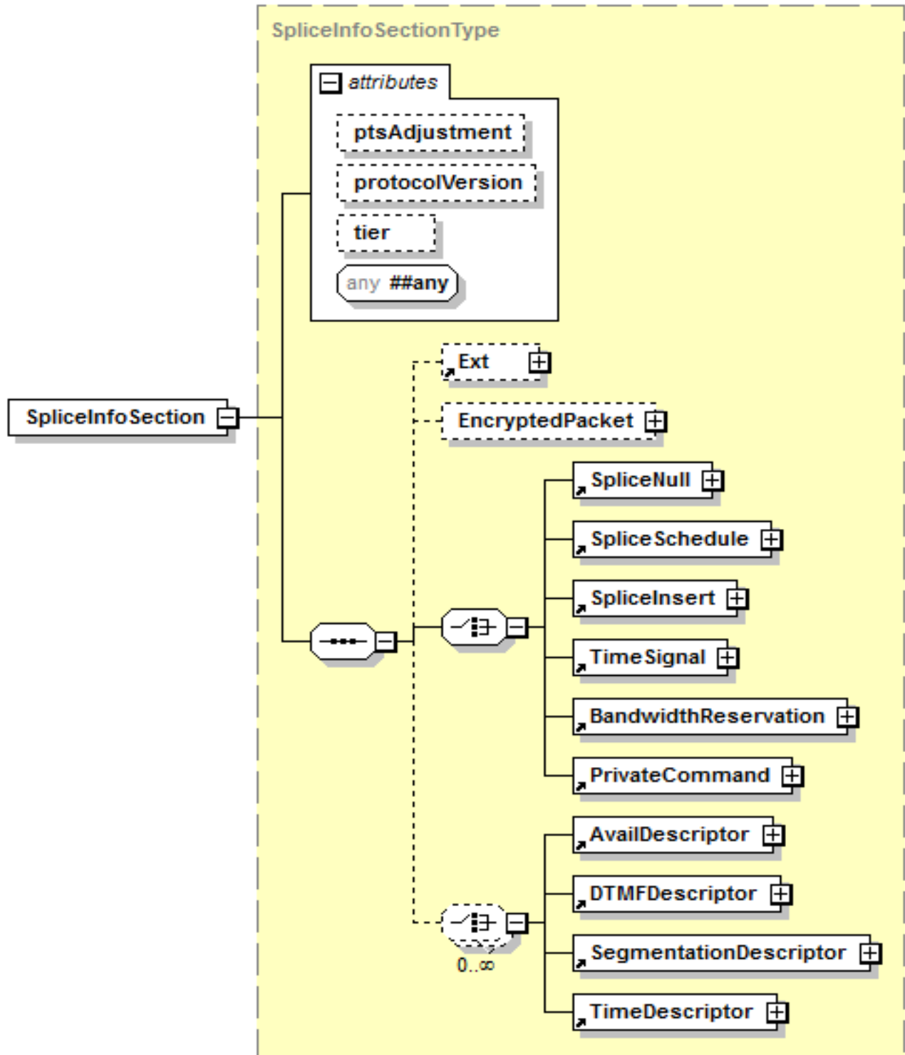
Figure 8-1. SpliceInfoSection
