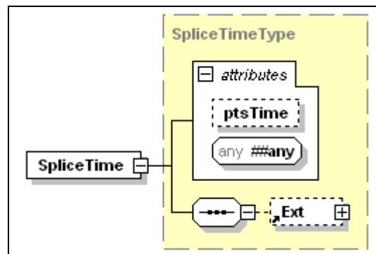
Figure 8-8. SpliceTime
