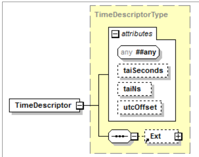
Figure 9-10. TimeDescriptor
