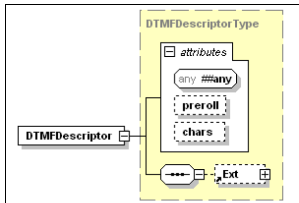
Figure 9-3. DTMFDescriptor
