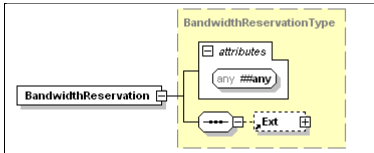
Figure 8-6. BandwidthReservation
