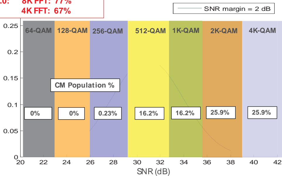
Figure 13. DOCSIS 3.1 US spectral efficiency with SNR operating margin = 2 dB
