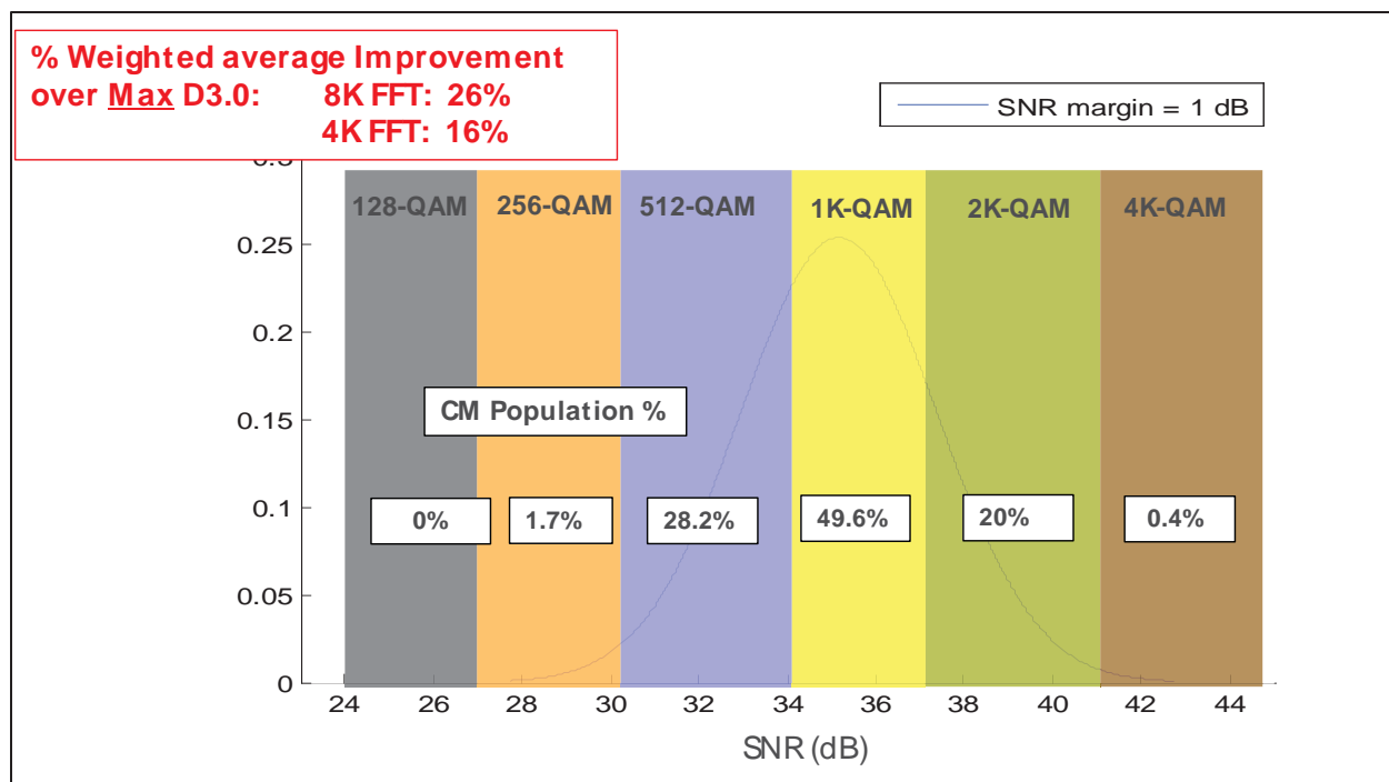
Figure 5. DOCSIS 3.1 DS spectral efficiency with SNR operating margin = 1 dB
