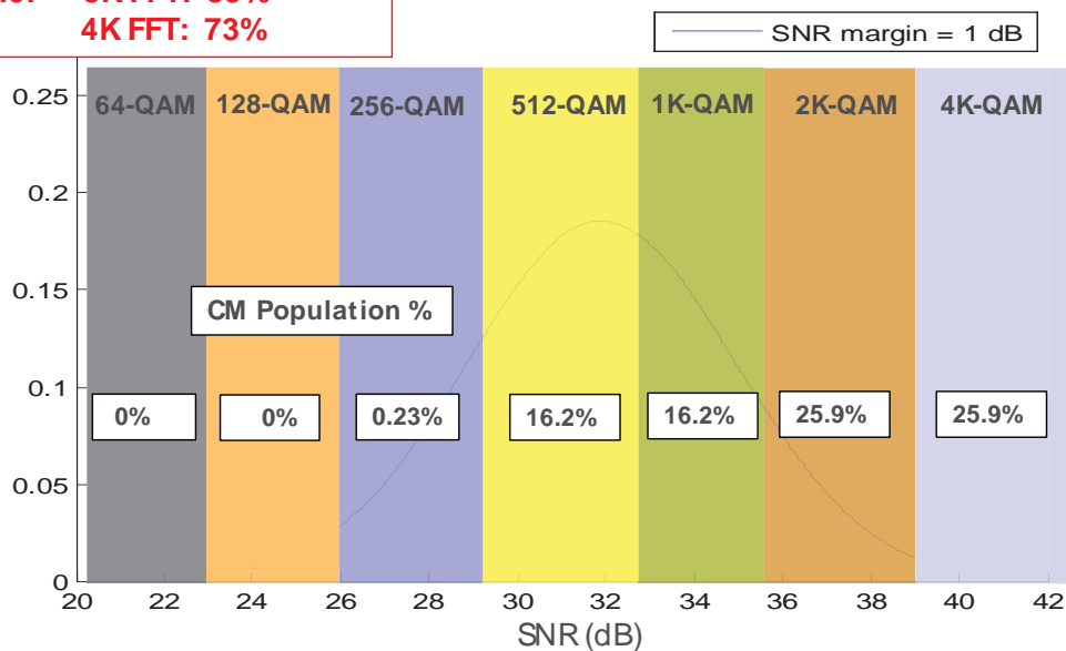
Figure 12. DOCSIS 3.1 US spectral efficiency with SNR operating margin = 1 dB
