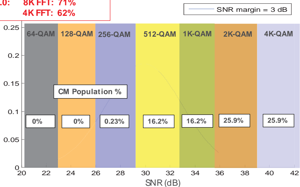
Figure 14. DOCSIS 3.1 US spectral efficiency with SNR operating margin = 3 dB
