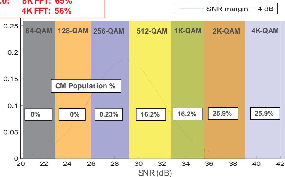
Figure 15. DOCSIS 3.1 US spectral efficiency with SNR operating margin = 4 dB
