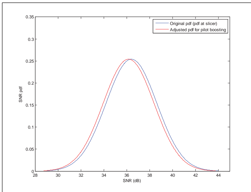
Figure 3. DS SNR distribution shifted by 0.25 dB to compensate for pilot boosting
