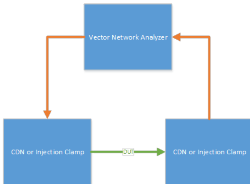
Figure 1 - Equipment Setup
