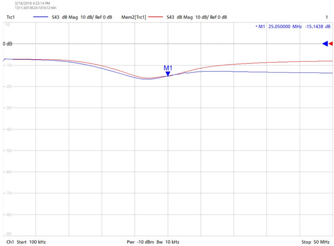
Figure 2 - S-Parameter of CM Filter (Blue Trace) vs No Filtering (Red Trace)
