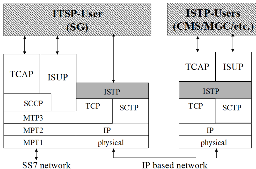
Figure 3. Protocol Distribution in IPCablecom Elements
