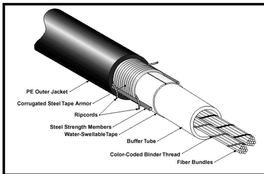
Figure 5 – Central Tube Cable (Bundled Fibers)
