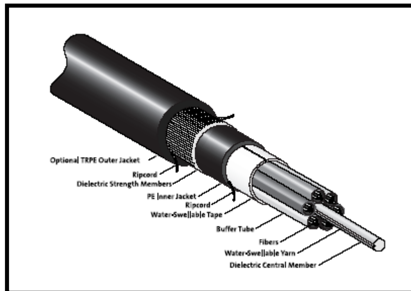
Figure 7 – All Dielectric Self Supporting (ADSS) Cable Design
