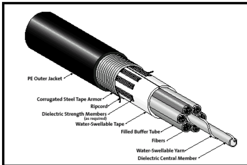
Figure 3 – Stranded Loose Tube Cable (Bundled Fibers)
