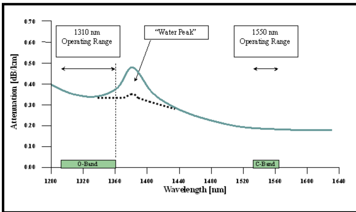
Figure 2 – Spectral Attenuation Curve for Optical Fiber
