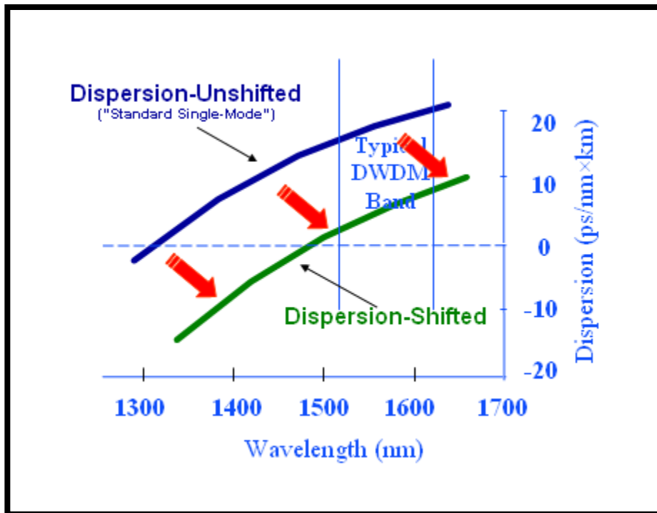
Figure 1 – Chromatic Dispersion in Optical Fiber
