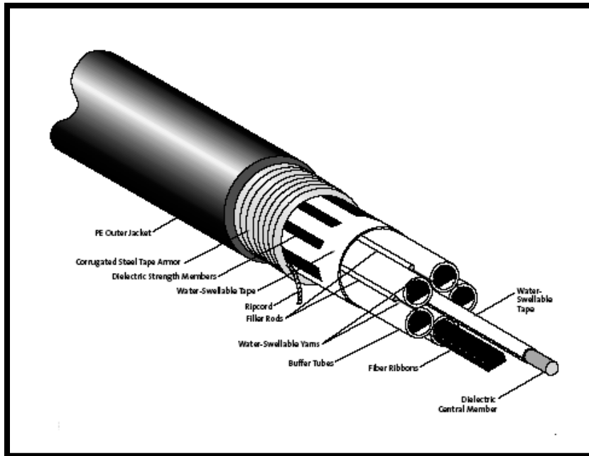
Figure 4 – Stranded Loose Tube Cable (Ribbonized Fibers)
