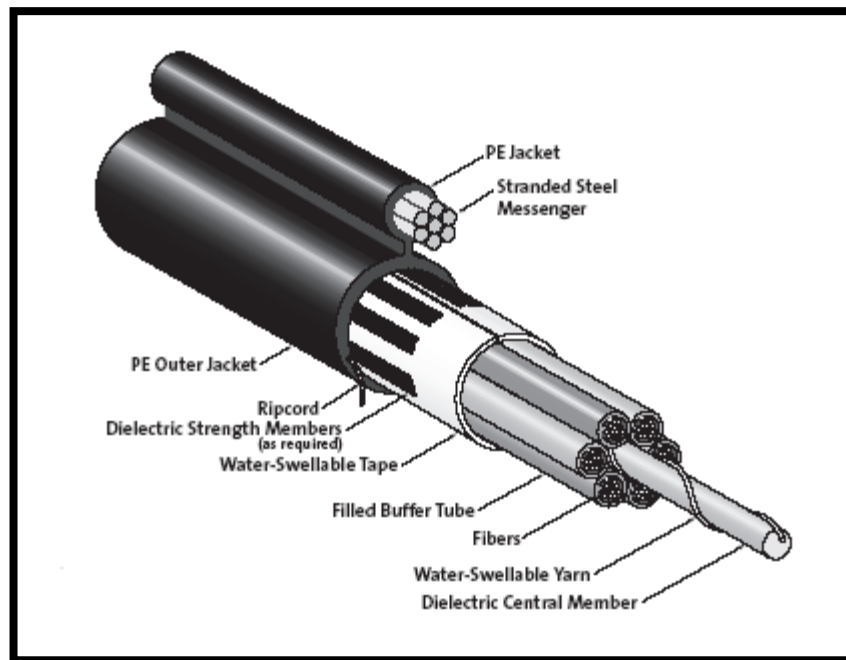
Figure 6 – Figure-8 Cable Design
