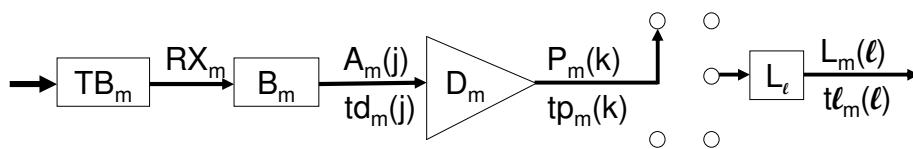
Figure 1: T-STD model
