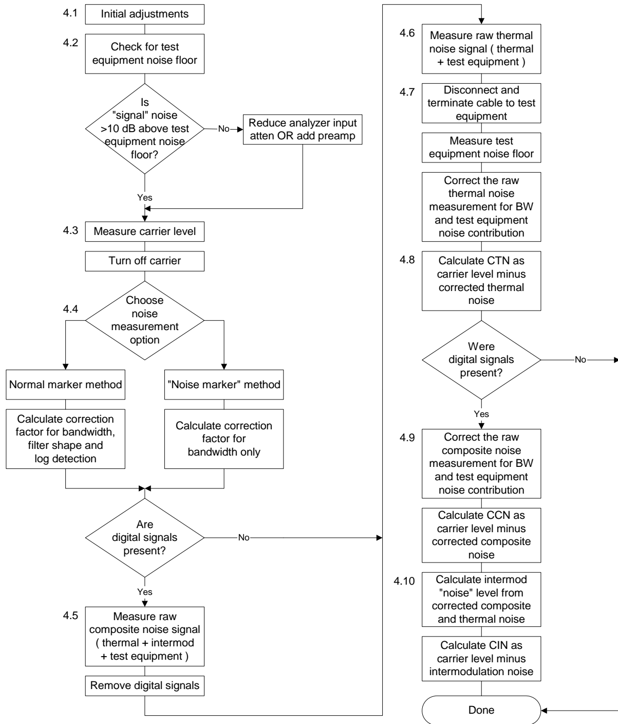
Figure 2: Flowchart for Carrier to Noise Measurements
