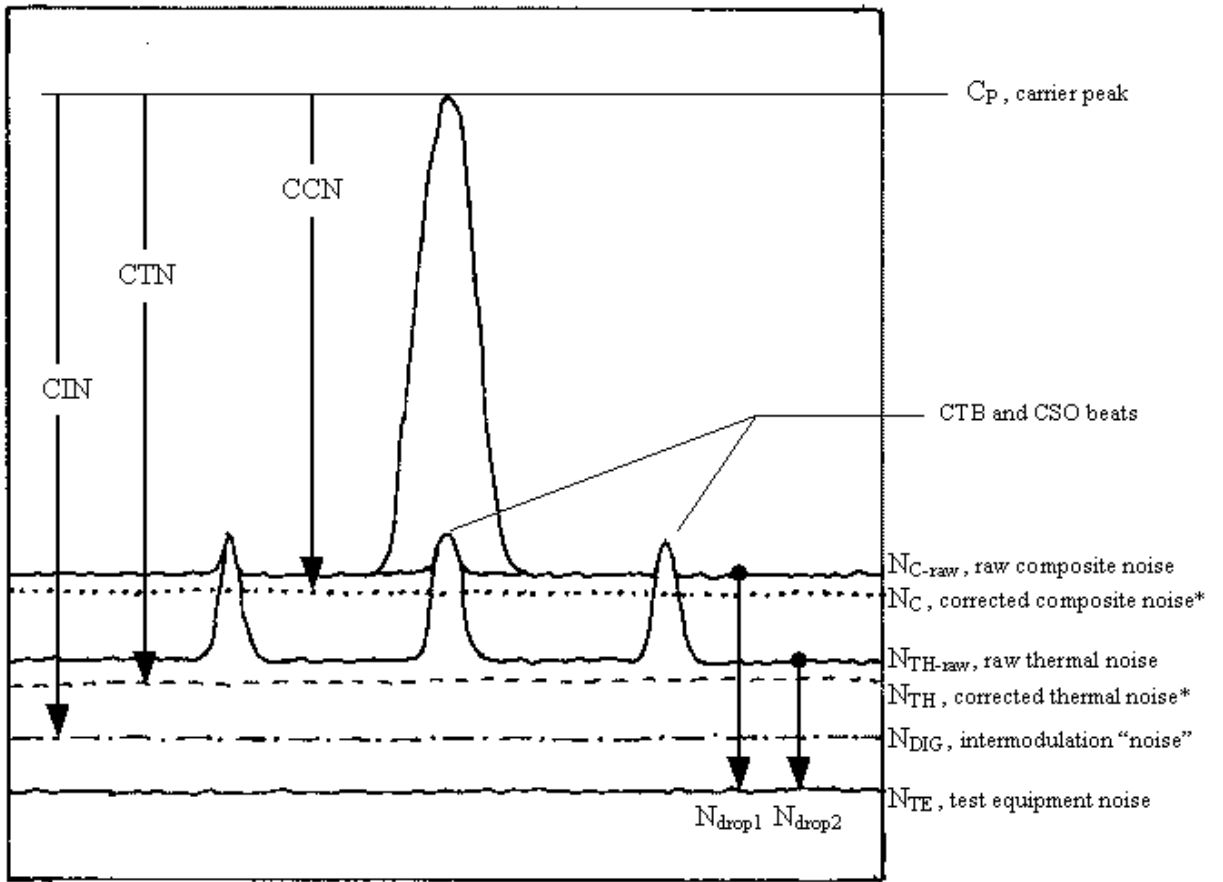
Figure 2 - Sketch of Noise Components
