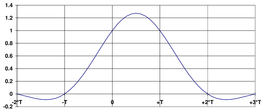
Figure 5-2 PRC Impulse Response
