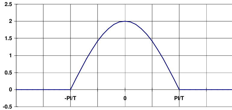
Figure 5-1 Frequency Response of PRC Filter (Linear Scale)
