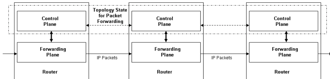
Figure 3 – Control and Forwarding Planes
