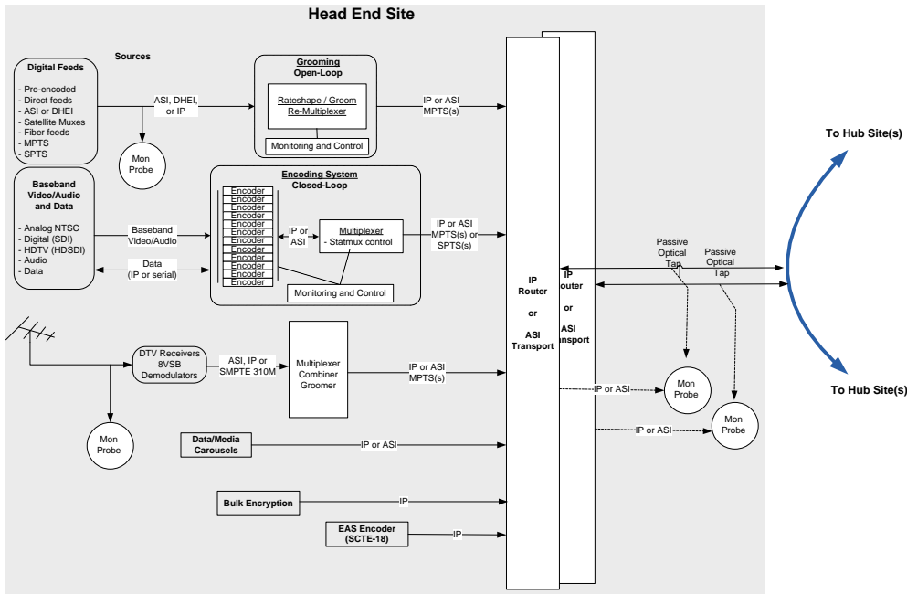
Figure 3: Redundant Connection to Core Transport System with Monitoring
