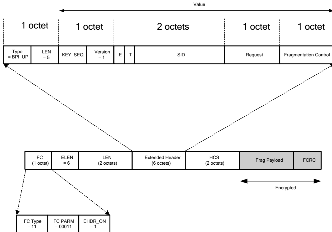
Figure 8-2 - Format of a DOCSIS MAC Fragmentation Frame with an Encrypted Payload
