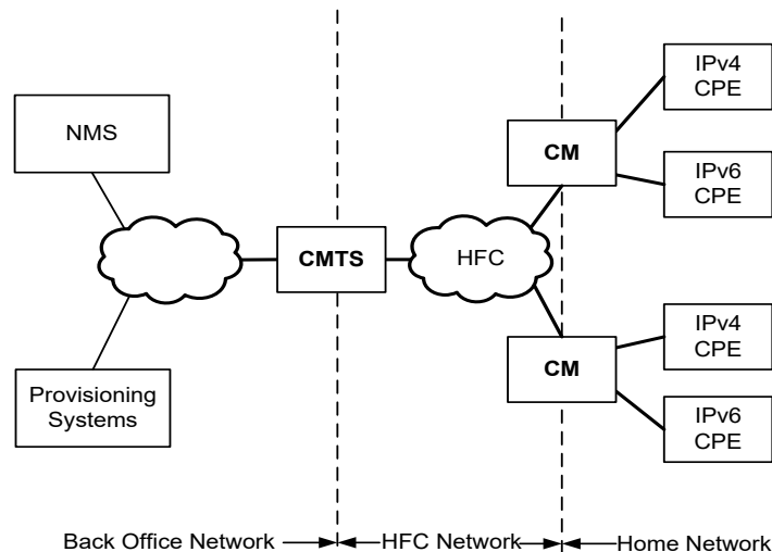
Figure 3-1 - The DOCSIS Network
