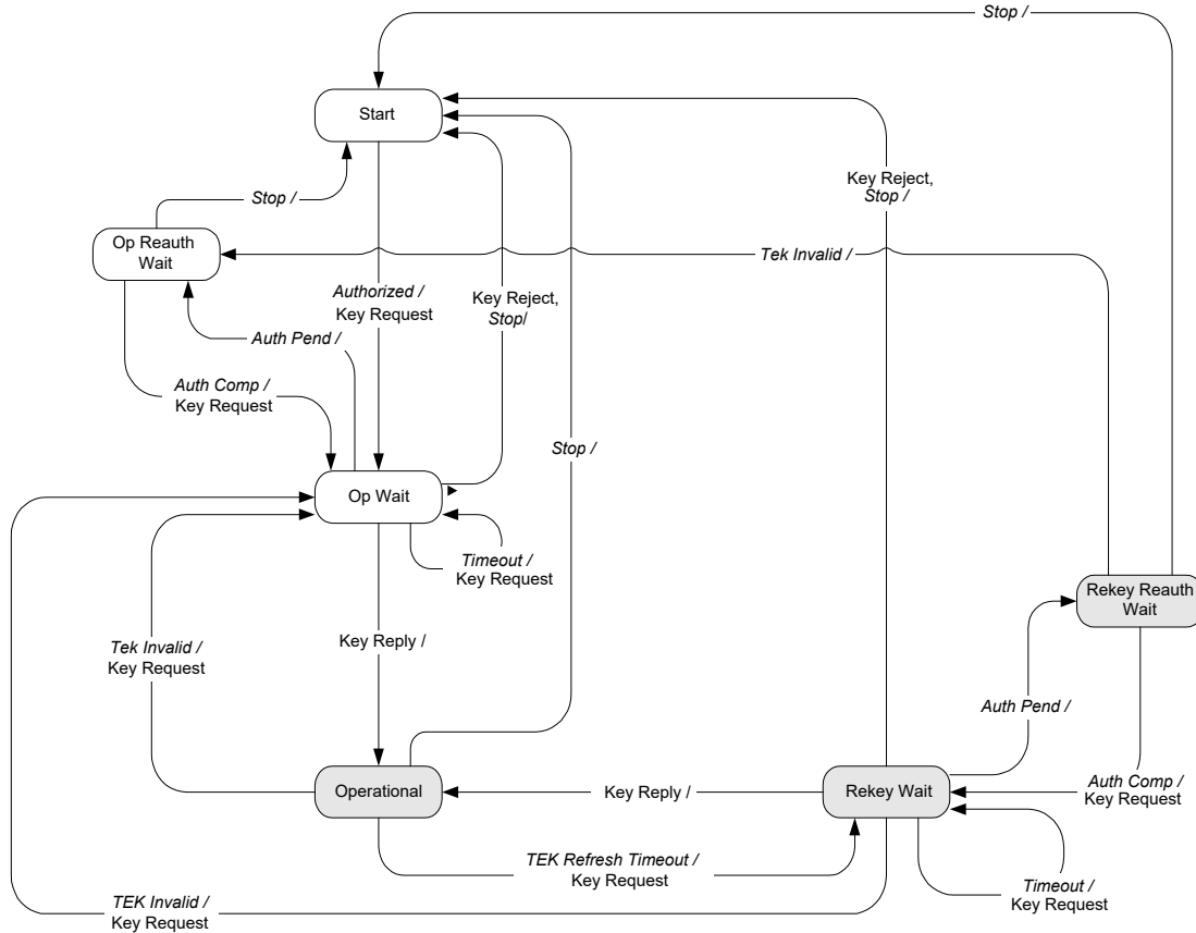
Figure 9-3 - TEK State Machine Flow Diagram
