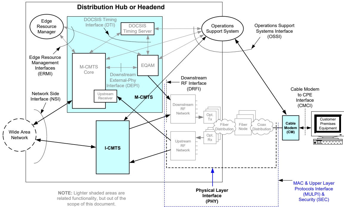
Figure 3-3 - Data-over-Cable Reference Architecture
