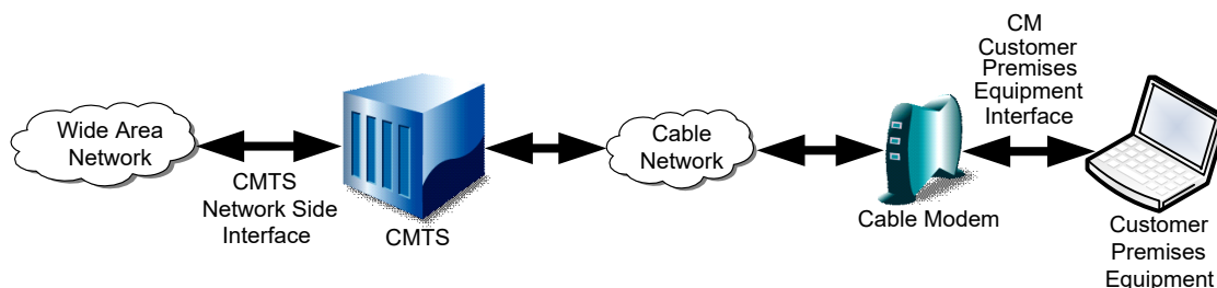
Figure 3-2 - Transparent IP Traffic Through the Data-Over-Cable System
