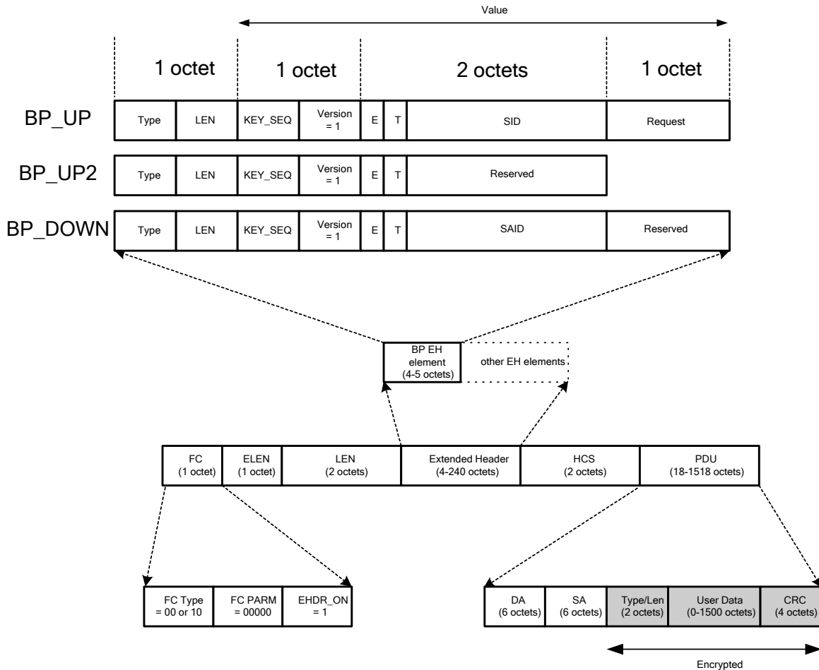
Figure 8-1 - Format of DOCSIS Variable-length PDU with Privacy EH Element
