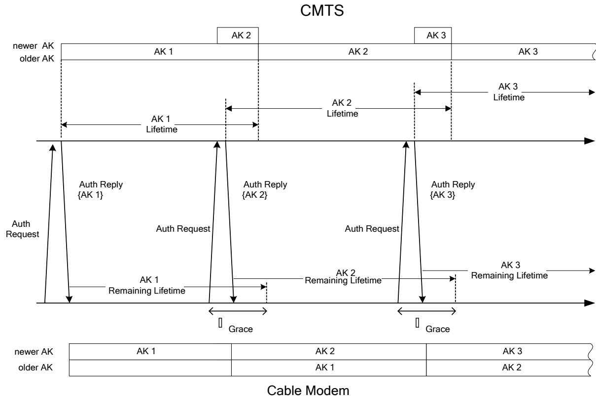
Figure 12-1 - Authorization Key Management in CMTS and CM
