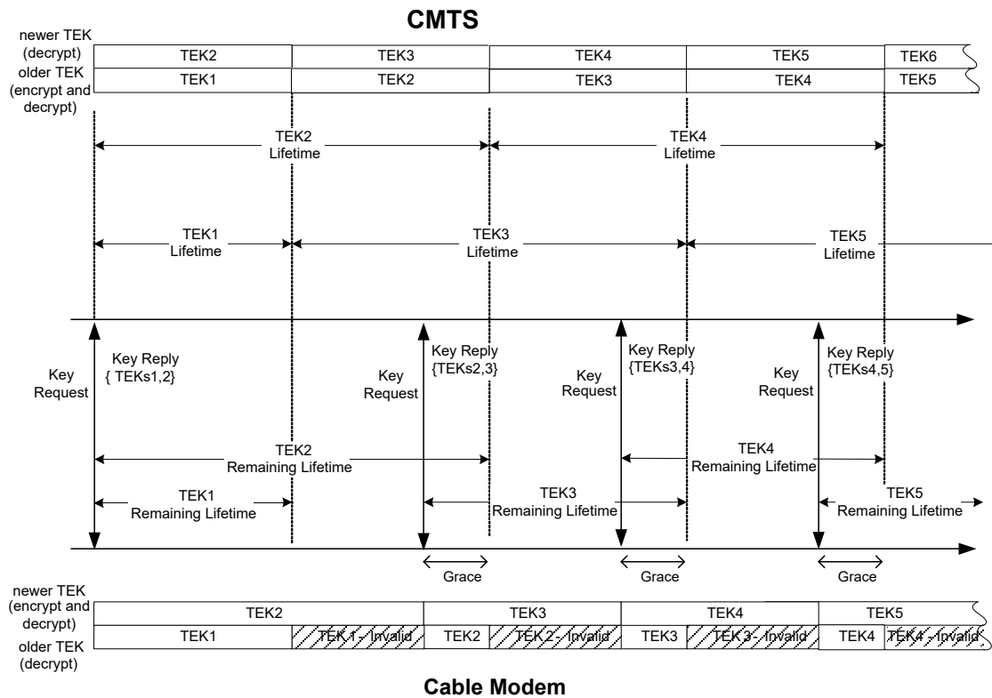
Figure 12-2 - TEK Management in CMTS and CM
