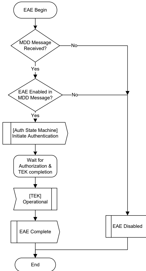
Figure 10-1 - EAE Signaling Flow Chart for CM
