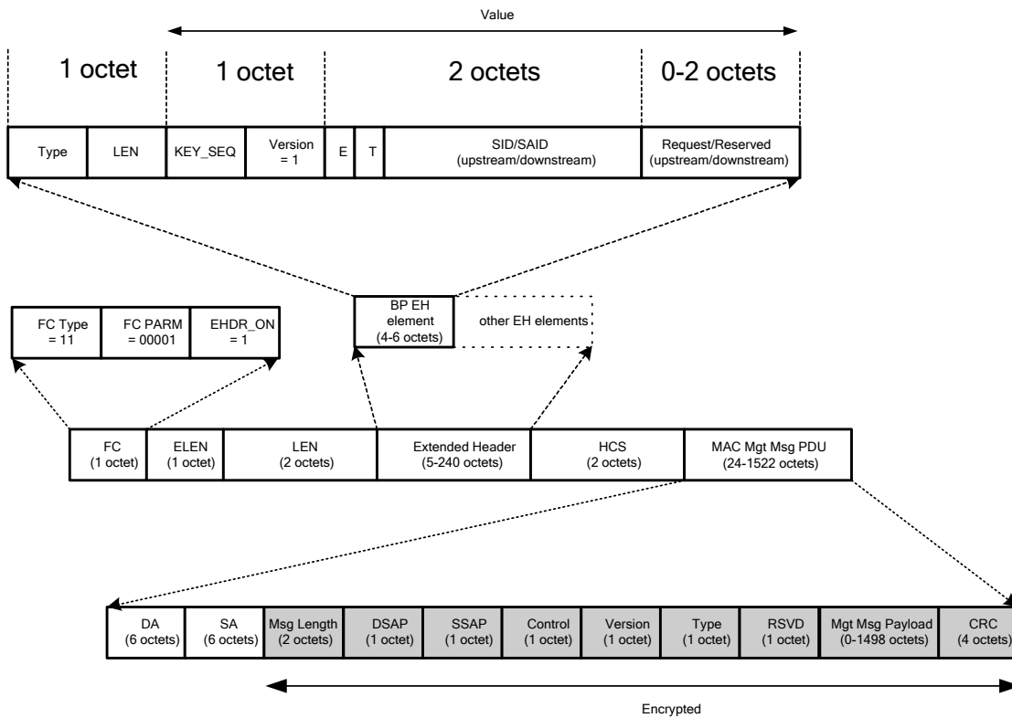
Figure 8-3 - Format of a DOCSIS MAC Management Message Frame with Encrypted Payload
