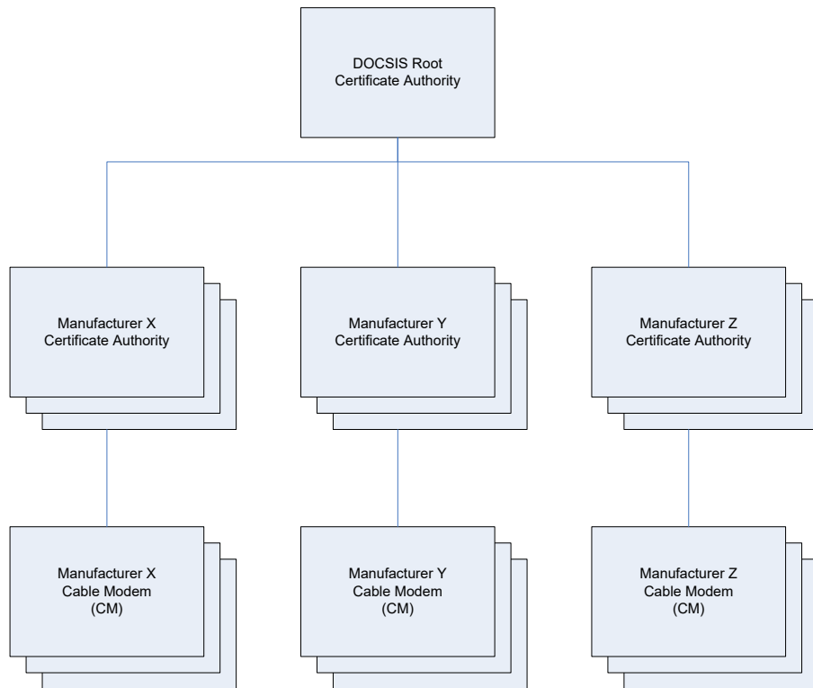
Figure 15-2 - The Distributed Model of the DOCSIS Certificate Management Architecture
