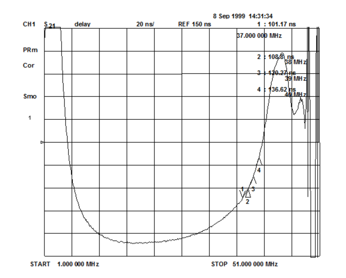
Figure 2 - Typical 5-40 MHz Reverse Path Group Delay Measurement
