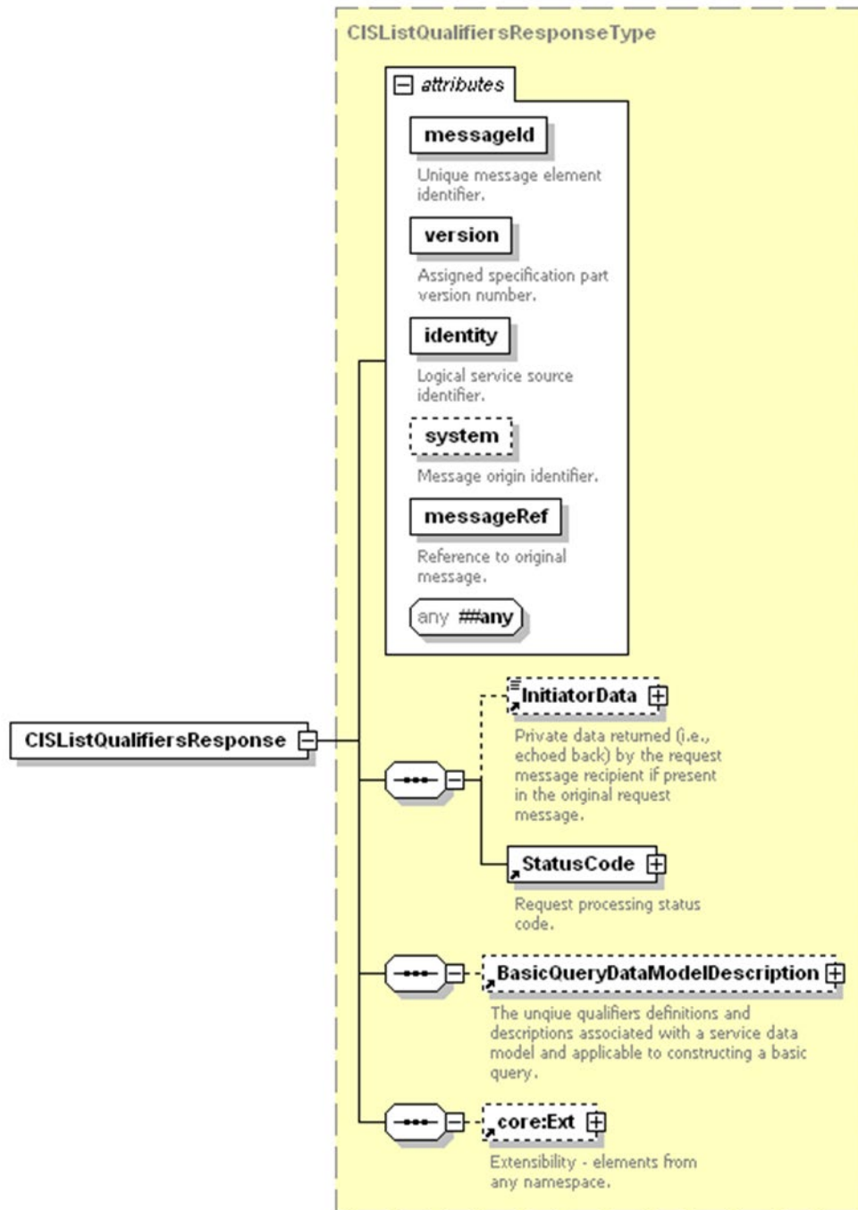
Figure 7 - CISListQualifiersResponse XML Schema
