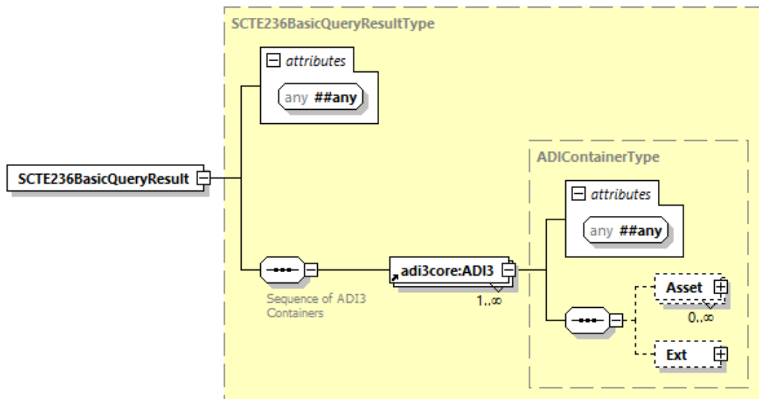
Figure 25 – SCTE 236 Metadata Data Model Connector XML Schema
