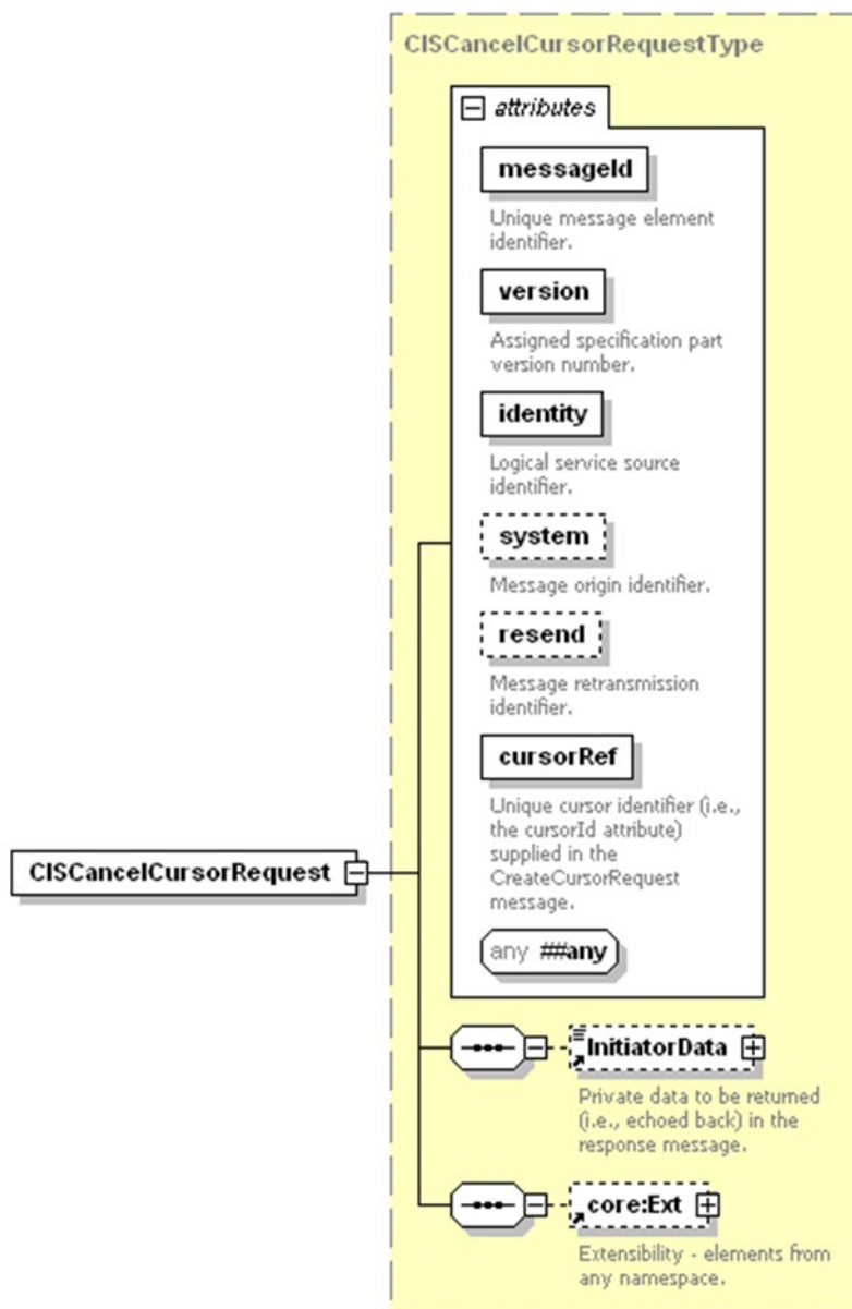
Figure 16 - CISCancelCursorRequest XML Schema
