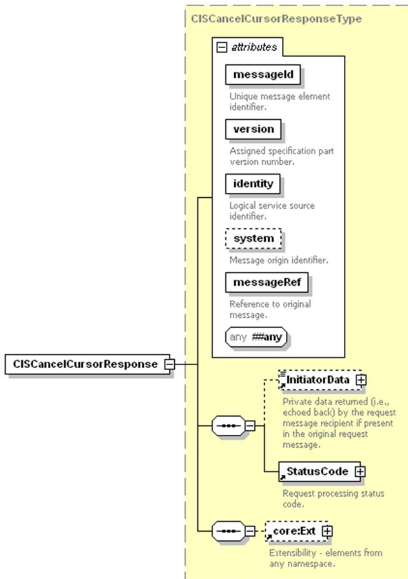
Figure 17 - CISCancelCursorResponse XML Schema
