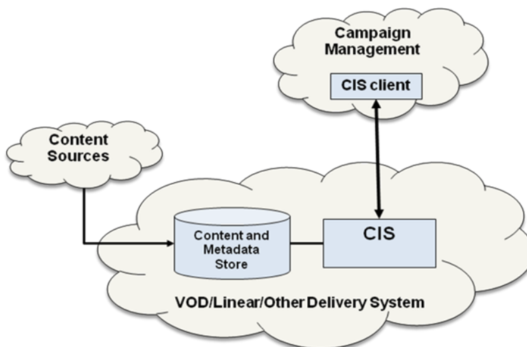
Figure 1 - CIS Content Storage
