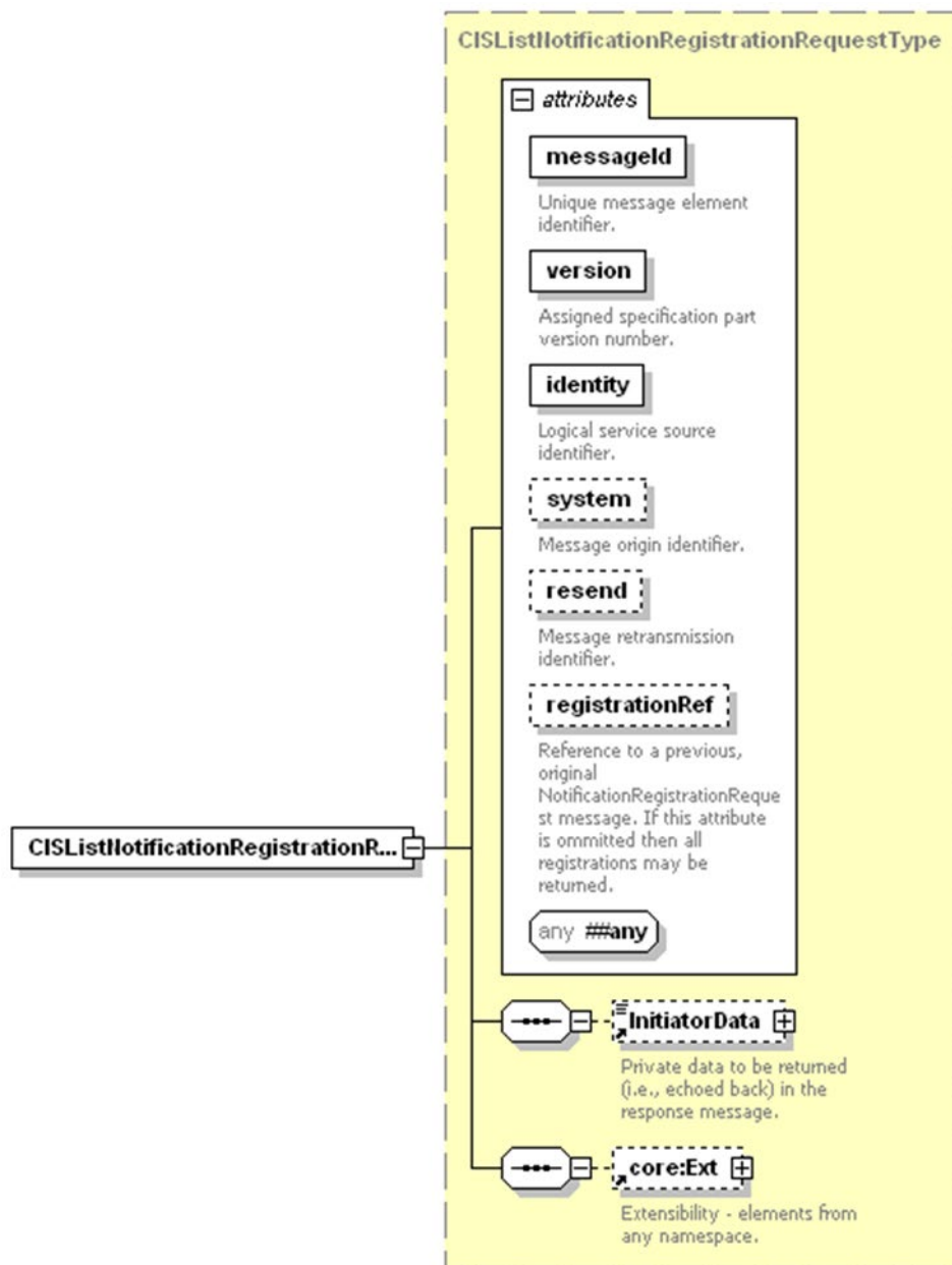
Figure 8 - CISListNotificationRegistrationRequest XML Schema
