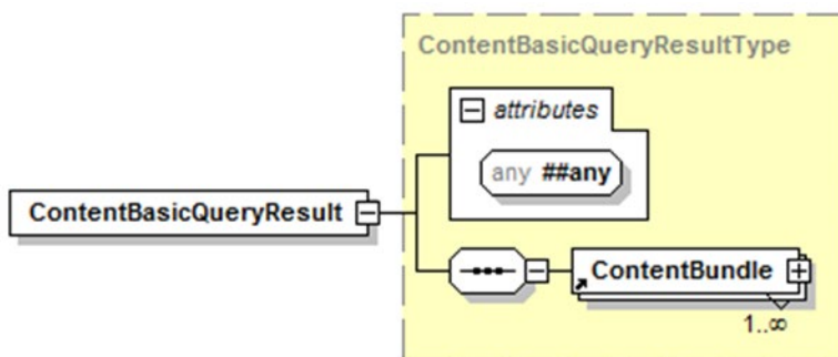
Figure 26 - Content Forecasting Data Model Connector XML Schema
