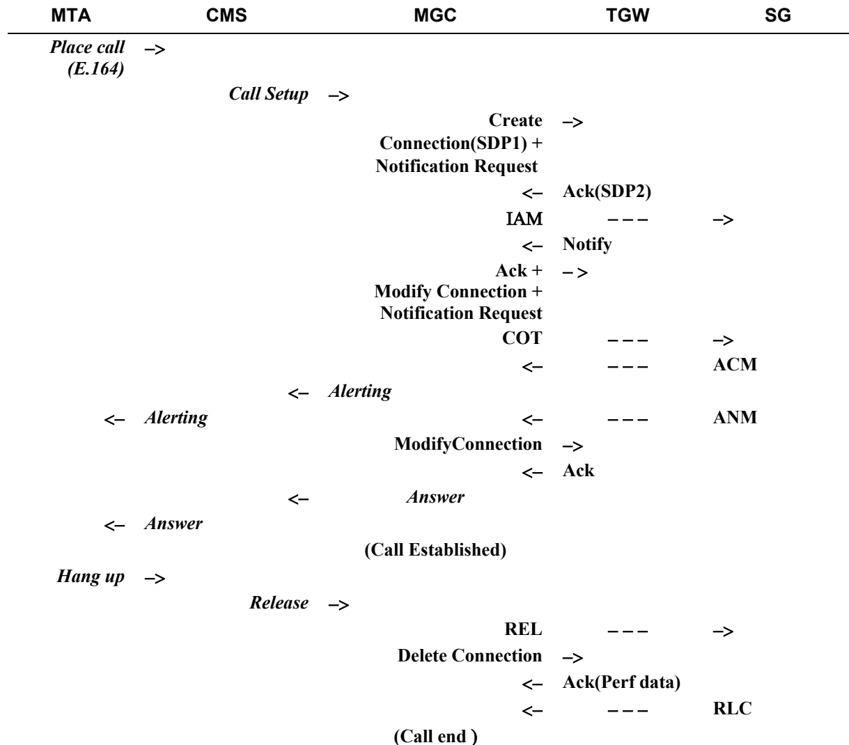
Figure 4 - MGCP Call Flow
