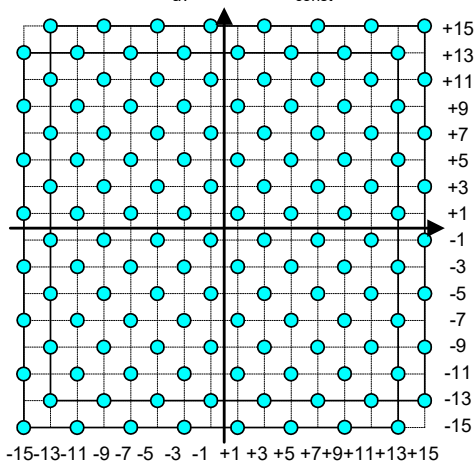
Figure 6–18 Symbol Constellations
