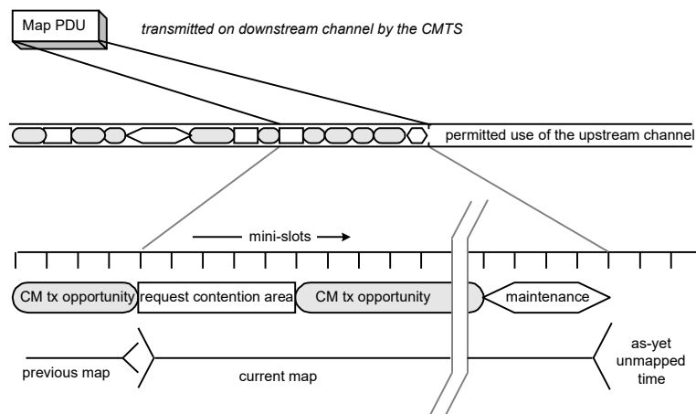
Figure 9–1 Allocation Map
