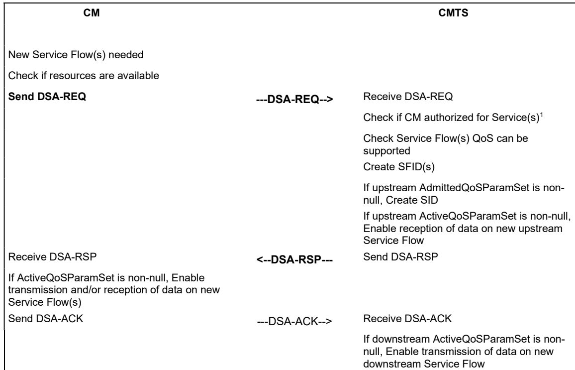
Figure 11–29 Dynamic Service Addition Initiated from CM
