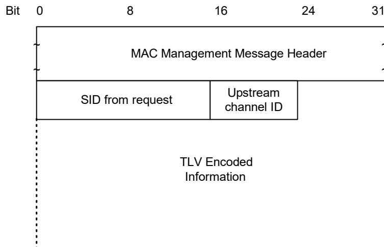
Figure 8–22 Ranging Response
