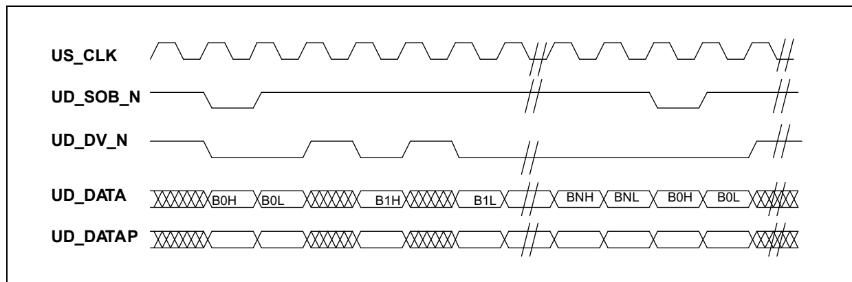
Figure H-4 Upstream Data Protocol
