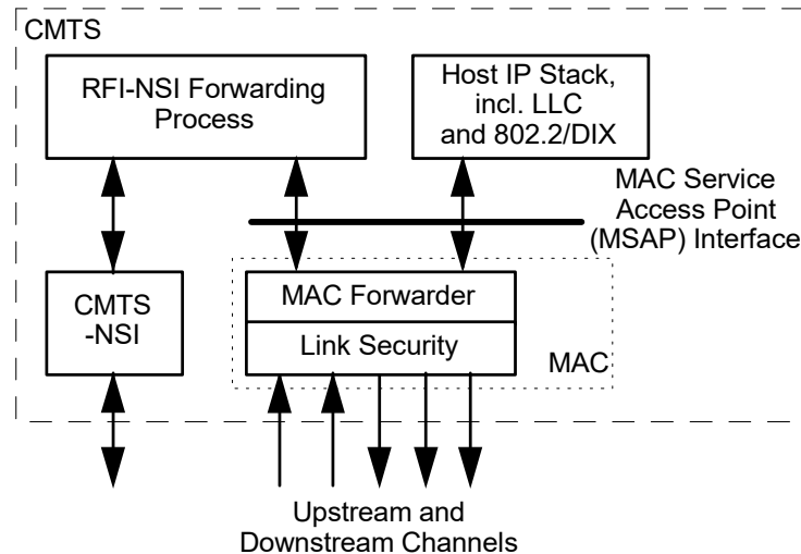
Figure 5–4 MAC Forwarder
