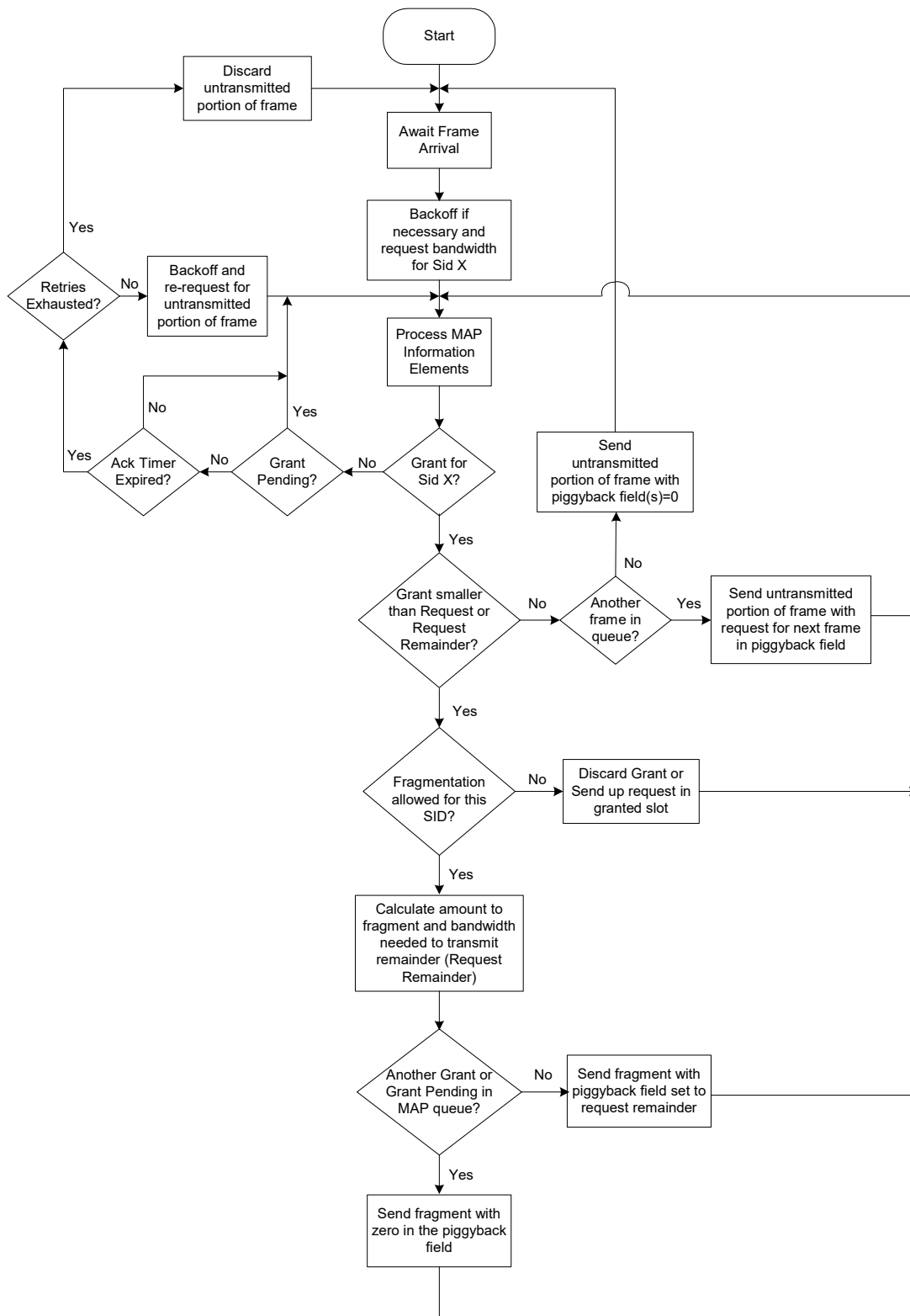
Figure 10–8 CM Fragmentation Flowchart
