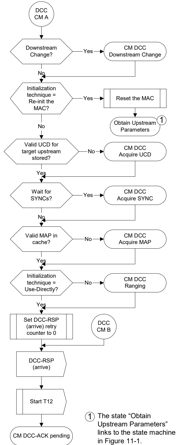
Figure 11-63 Dynamically Channels: CM View Part 2
