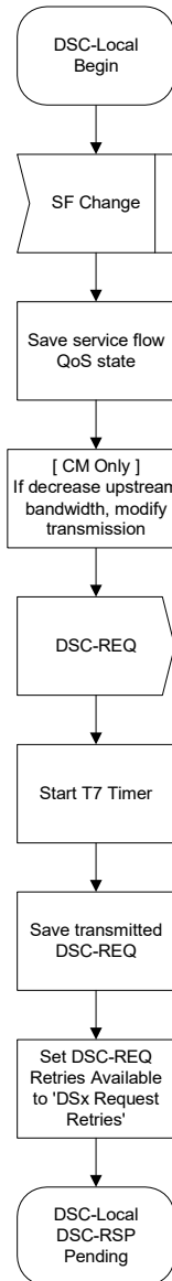
Figure 11–42 DSC—Locally Initiated Transaction Begin State Flow Diagram
