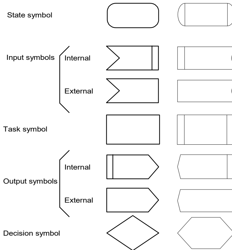
Figure 11-2 SDL Notation
