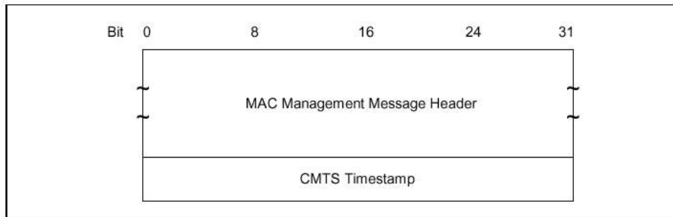
Figure F-3 Format of Packet PDU Following the Timing Header
