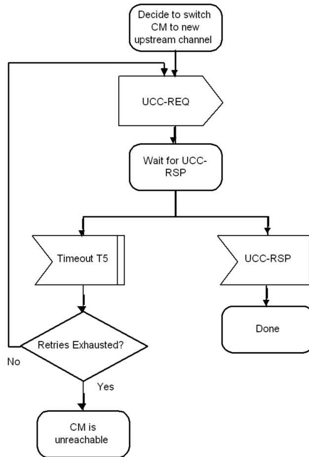
Figure 11–18 Changing Upstream Channels: CMTS View
