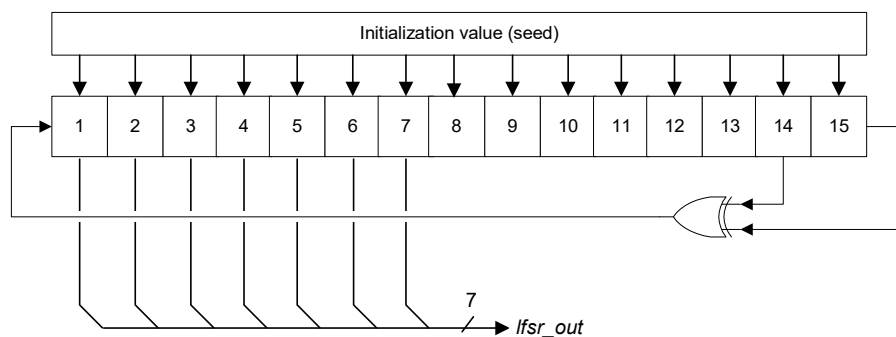
Figure 6–27 Code Hopping Random Number Generator
