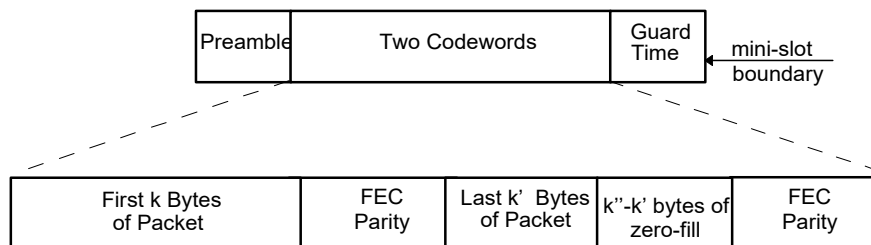
Figure 6–4 Example Frame Structures with Flexible Burst Length Mode
