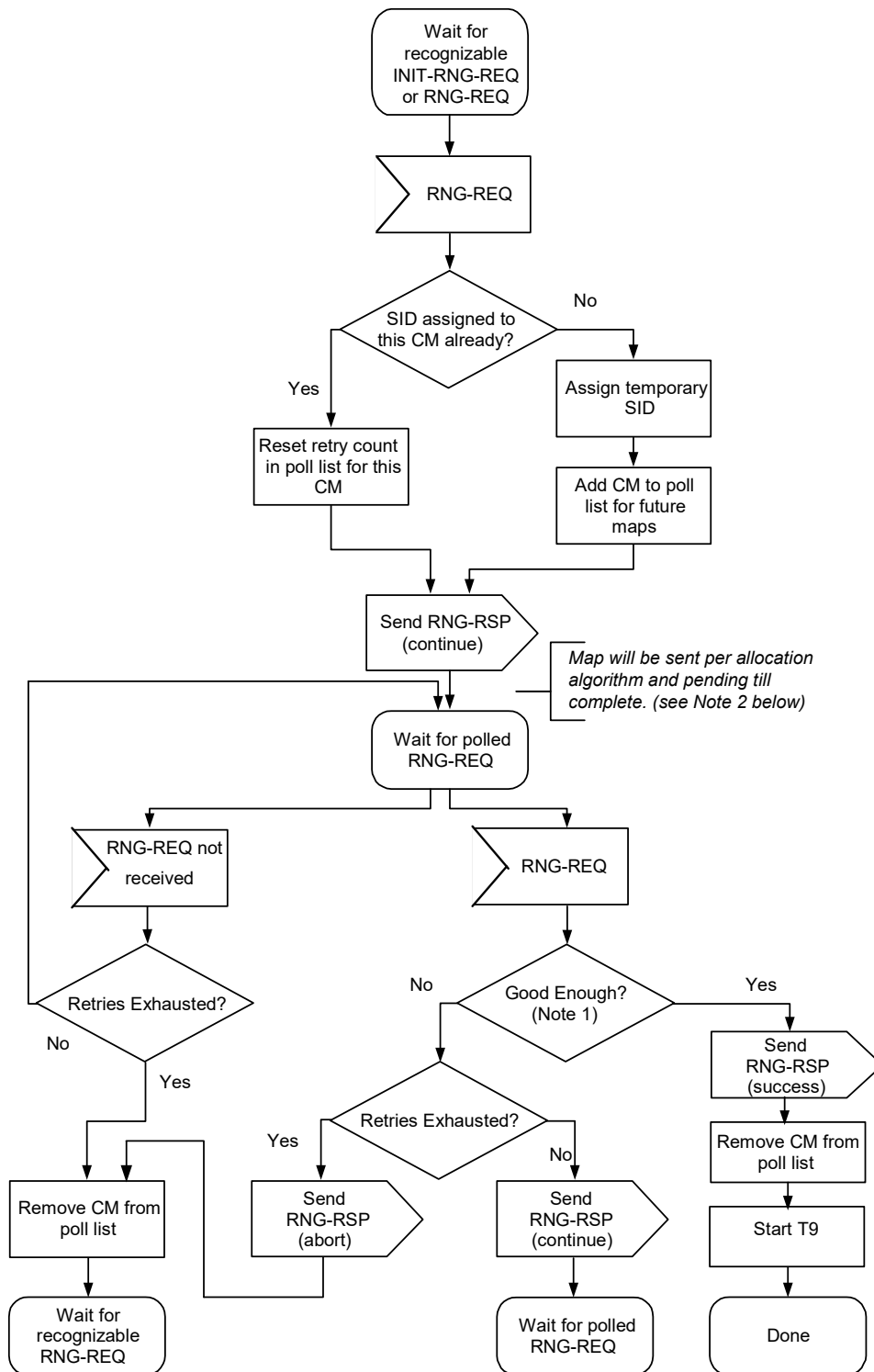
Figure 11–8 Initial Ranging - CMTS
