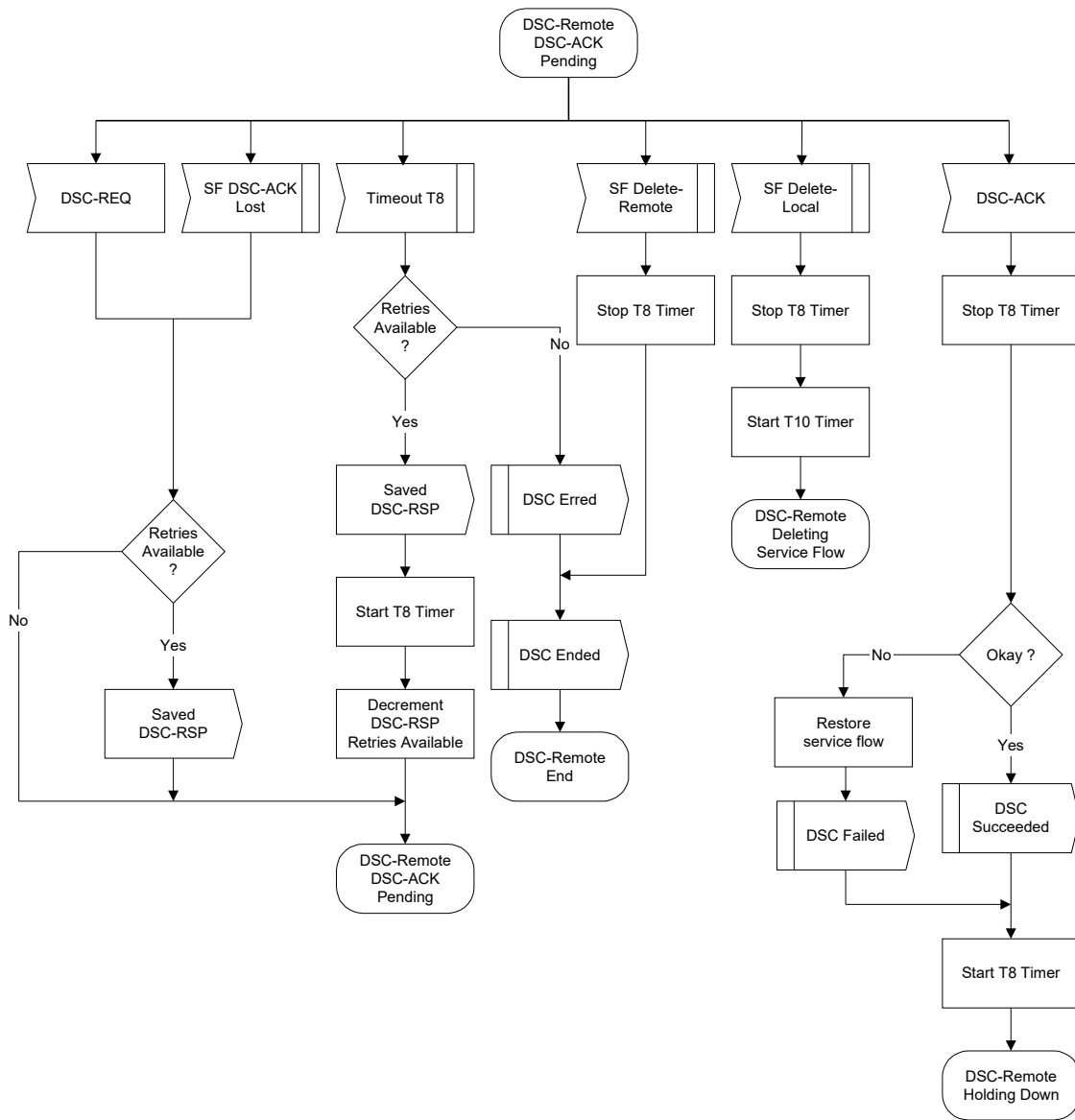
Figure 11–48 DSC—Remotely Initiated Transaction DSC-ACK Pending State Flow Diagram
