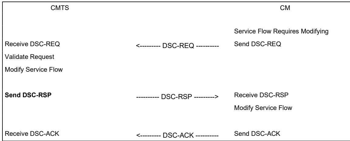
Figure 11–40 CM-Initiated DSC
