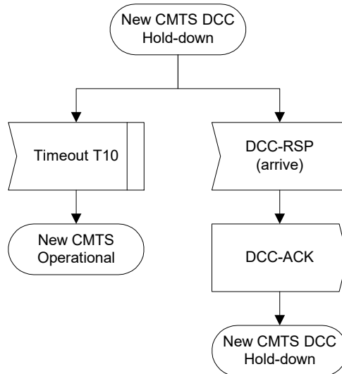
Figure 11-61 Dynamically Changing Channels: CMTS View Part 4
