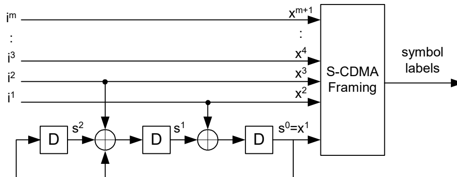
Figure 6–8 Convolutional encoder
