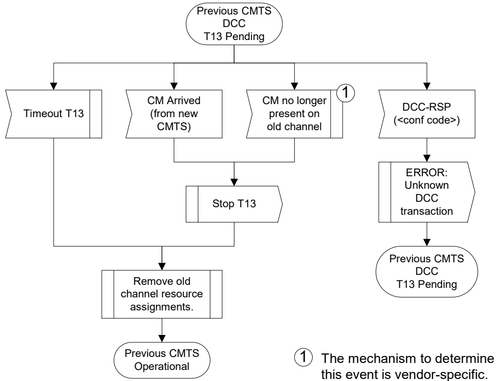
Figure 11–60 Dynamically Changing Channels: CMTS View Part 3
