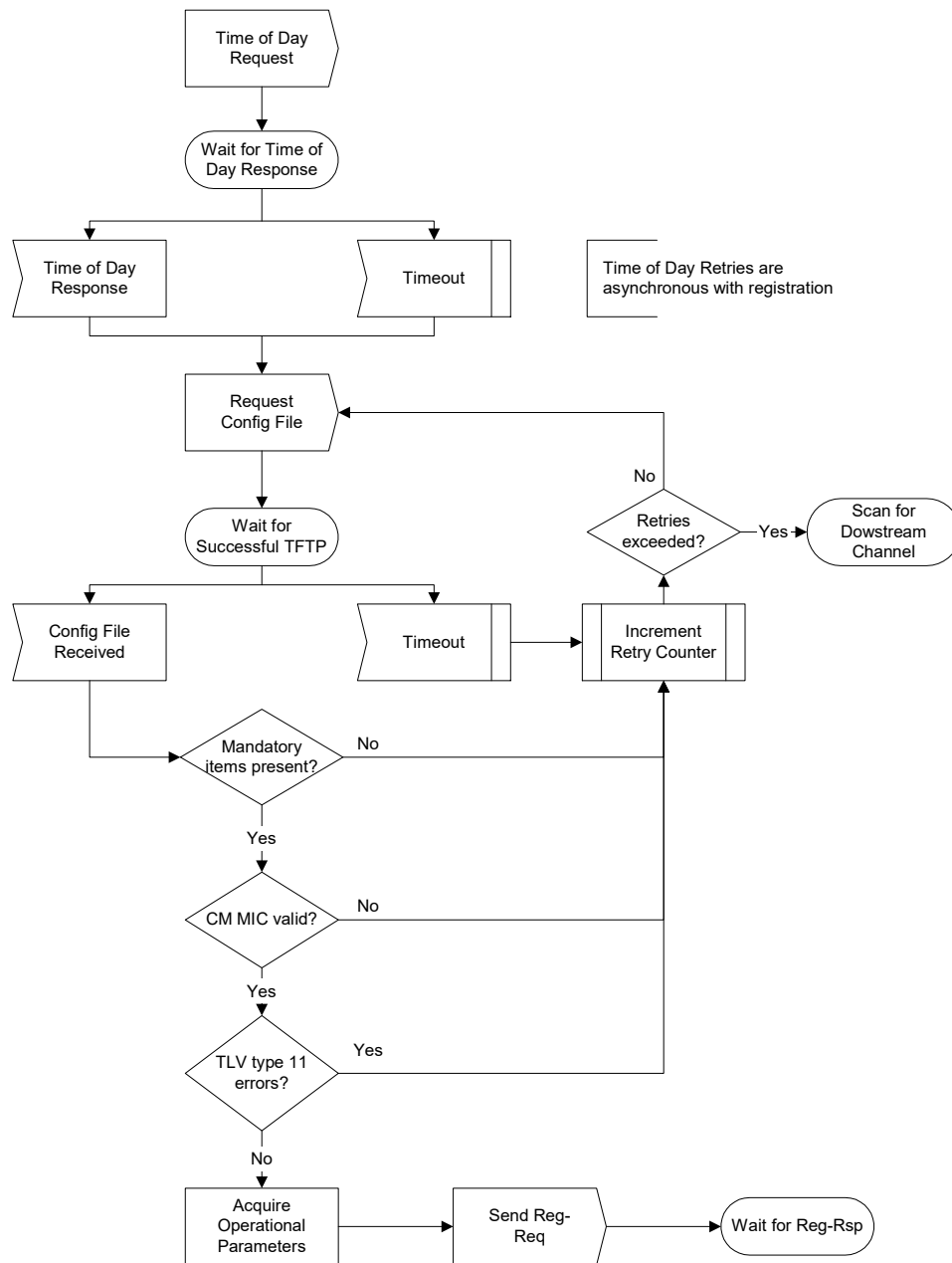
Figure 11–12 Registration — CM
