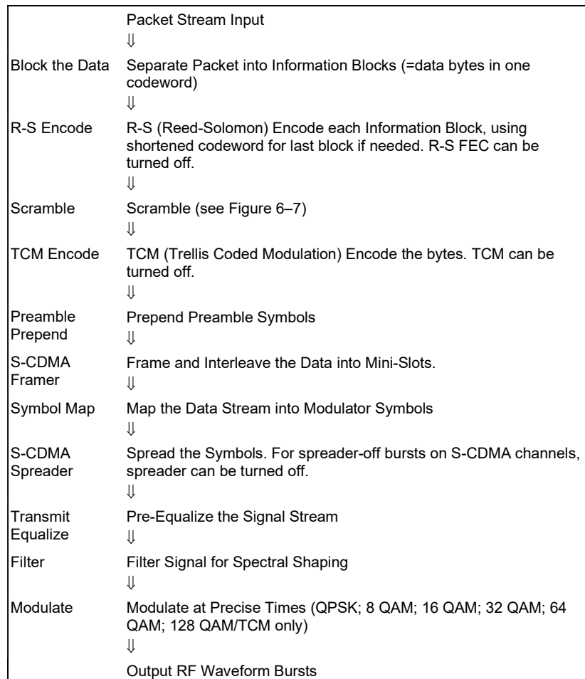
Figure 6–3 S-CDMA Upstream Transmission Processing
