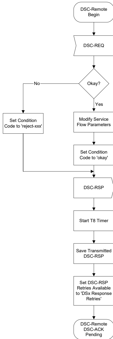
Figure 11–47 DSC—Remotely Initiated Transaction Begin State Flow Diagram
