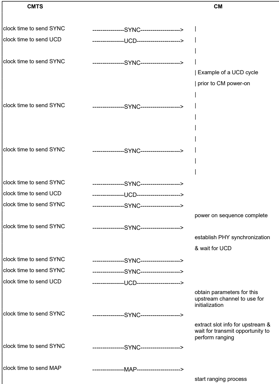
Figure 11-4 Message Flows During Scanning and Upstream Parameter Acquisition
