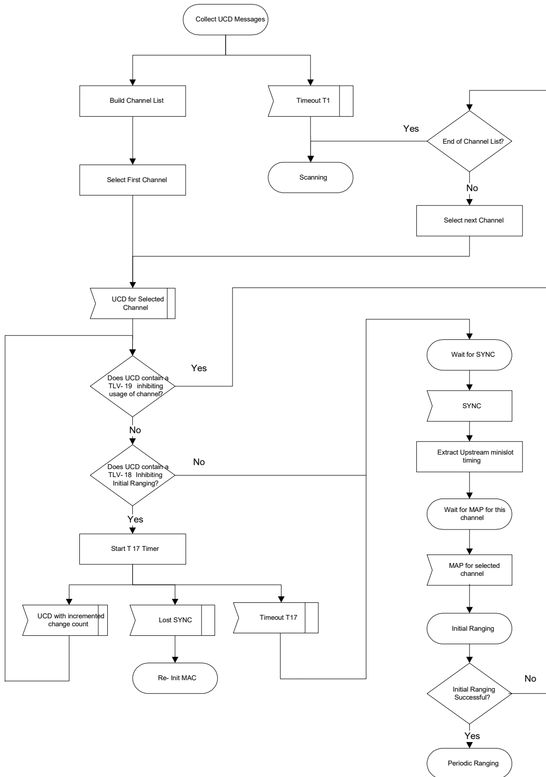
Figure 11-3 Obtaining Upstream Parameters
