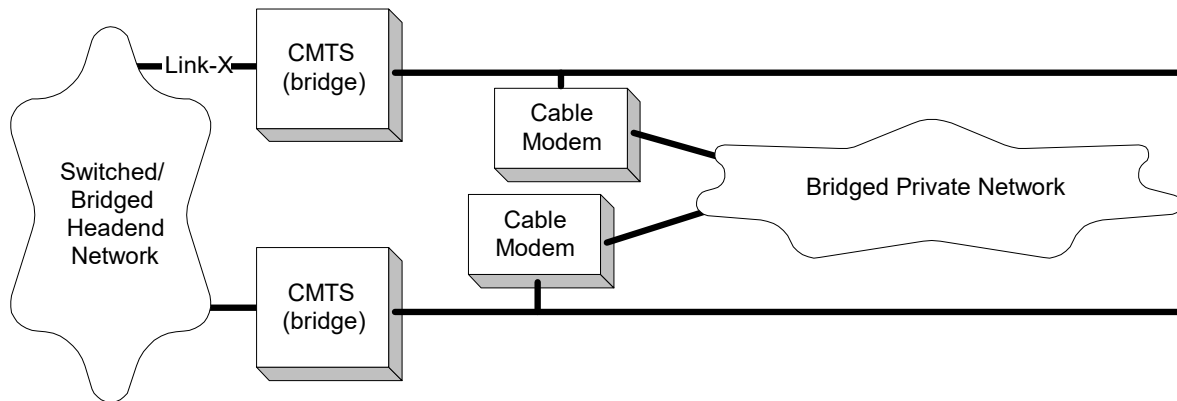
Figure E-2 Spanning Tree Across CMTSes
