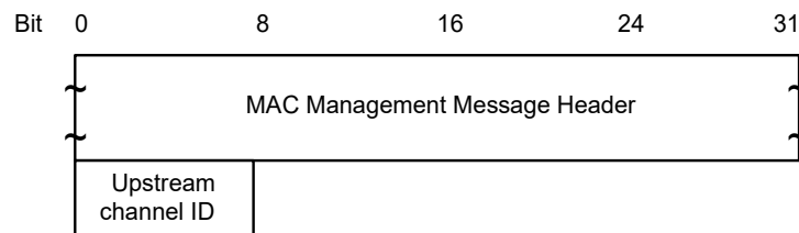
Figure 8–28 Upstream Channel Change Request
