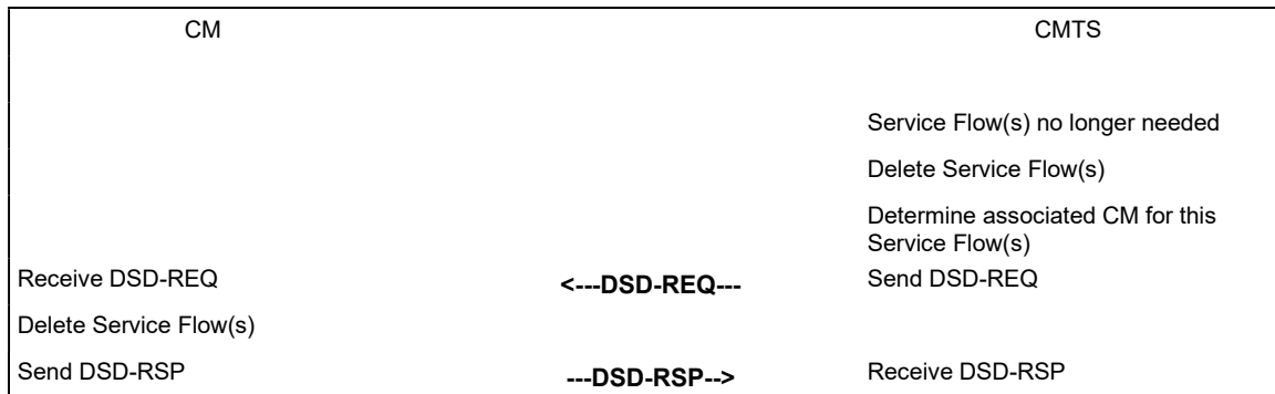
Figure 11–52 Dynamic Service Deletion Initiated from CMTS
