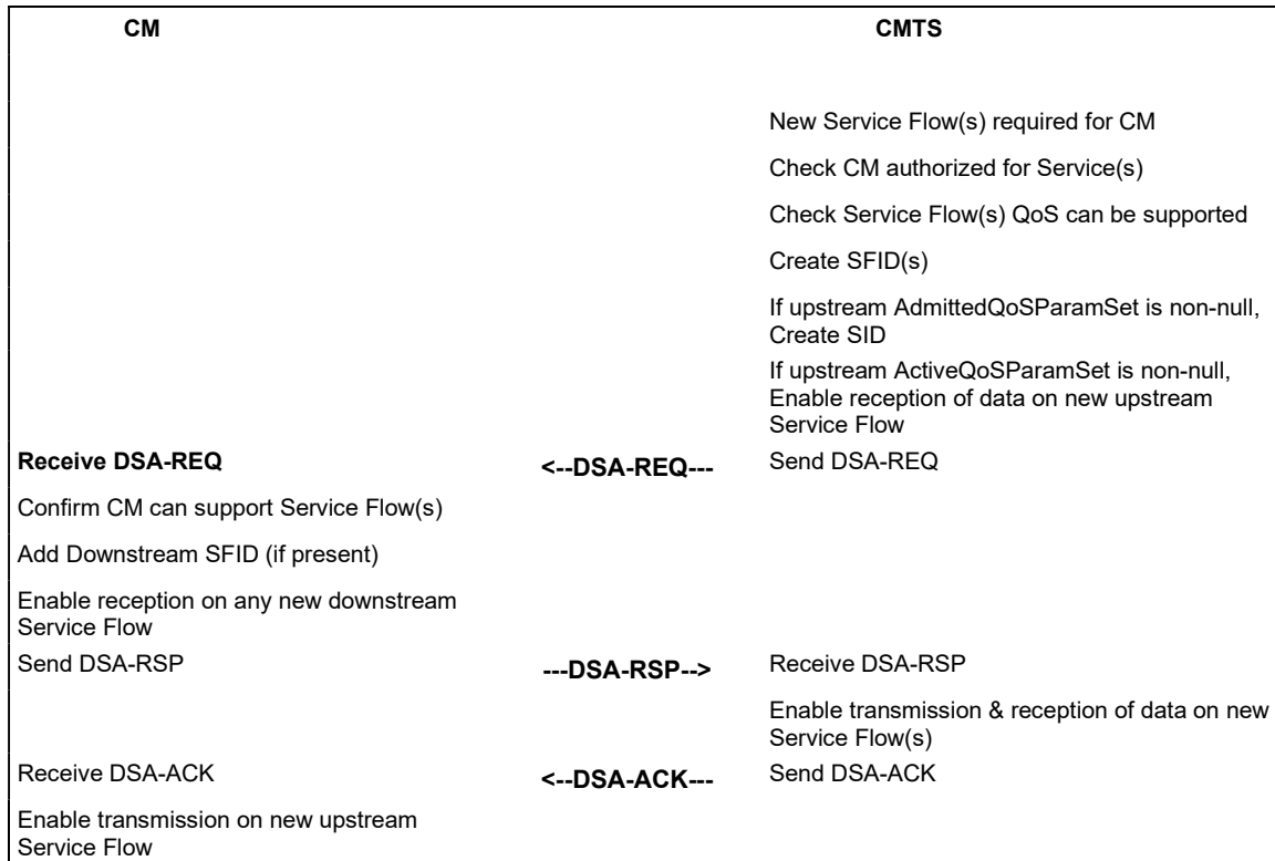
Figure 11–30 Dynamic Service Addition Initiated from CMTS
