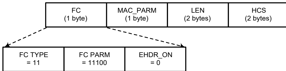
Figure 8–11 Concatenation MAC Header Format
