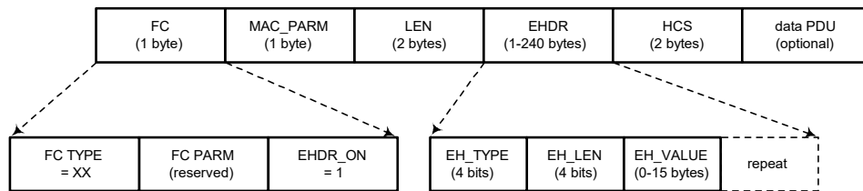
Figure 8–12 Extended MAC Format
