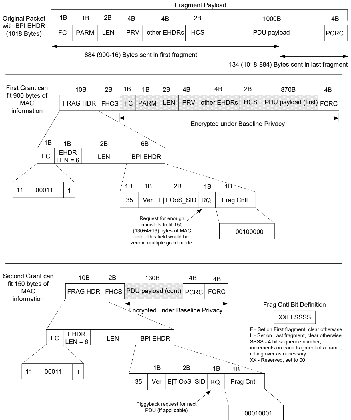
Figure 10-9 Example of Fragmenting a Single Packet
