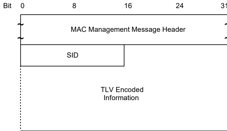
Figure 8–25 Registration Request
