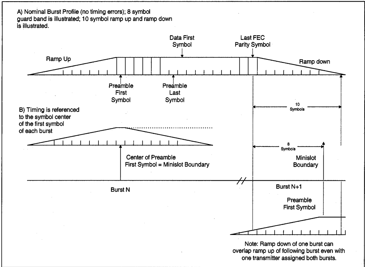
Figure 6-29 Nominal TDMA Burst Timing
