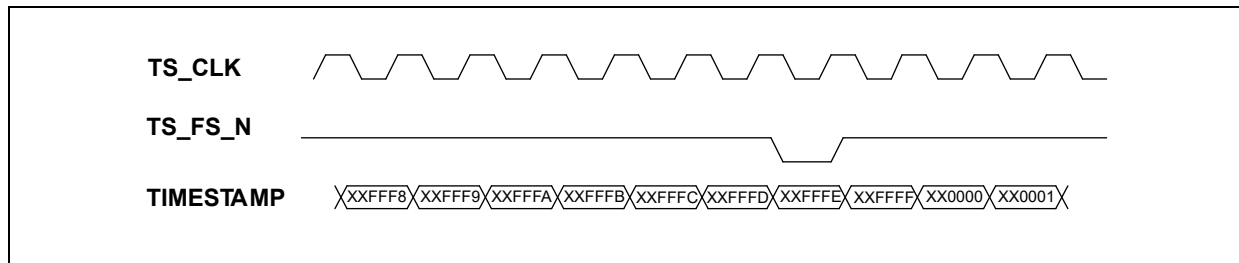
Figure H-5 Counter Synchronization
