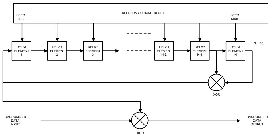
Figure 6–7 Scrambler Structure
