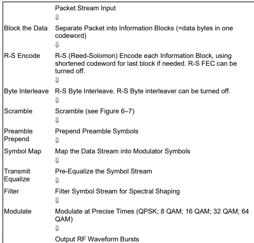
Figure 6-2 TDMA Upstream Transmission Processing
