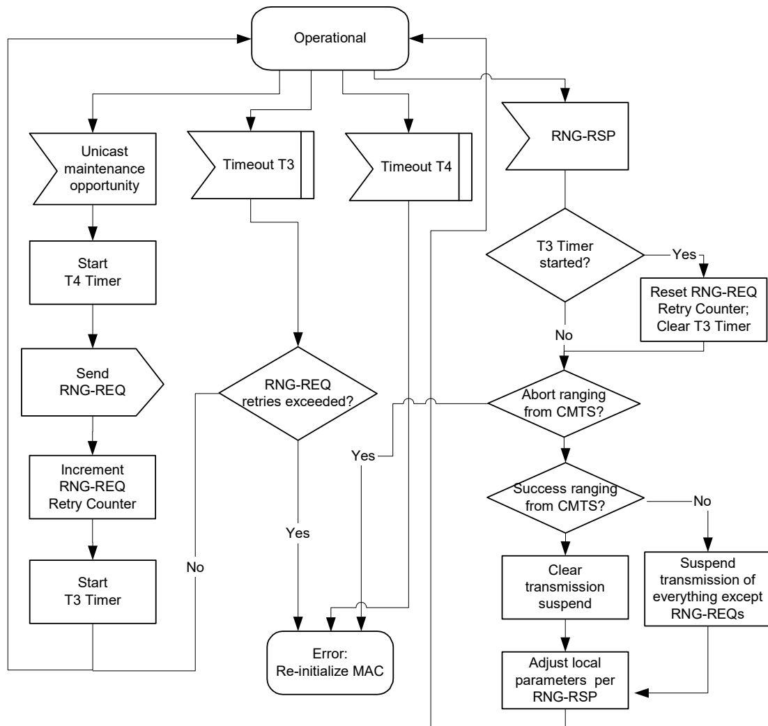
Figure 11–17 Periodic Ranging - CM View
