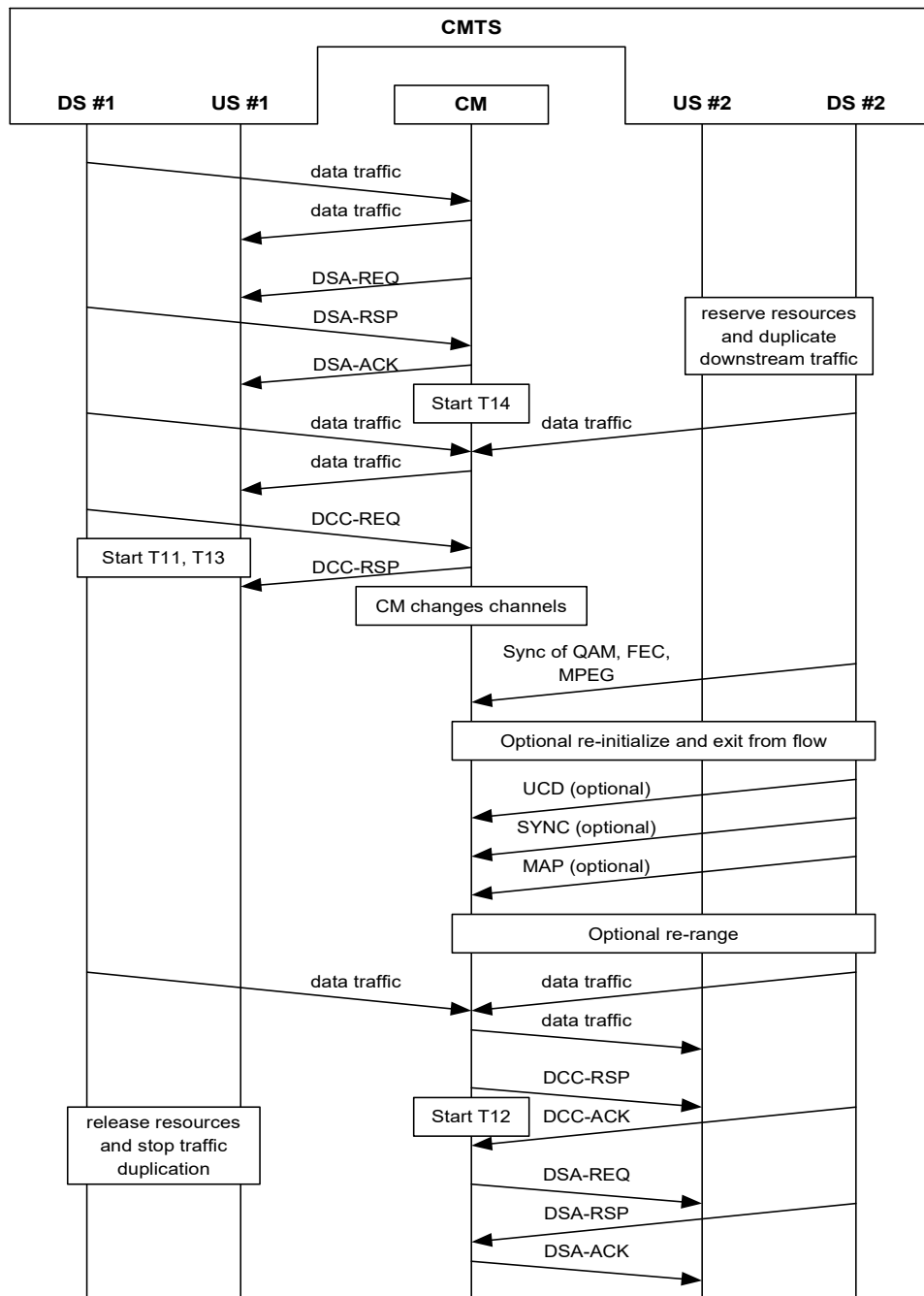
Figure 11–66 DCC Example Operational Flow
