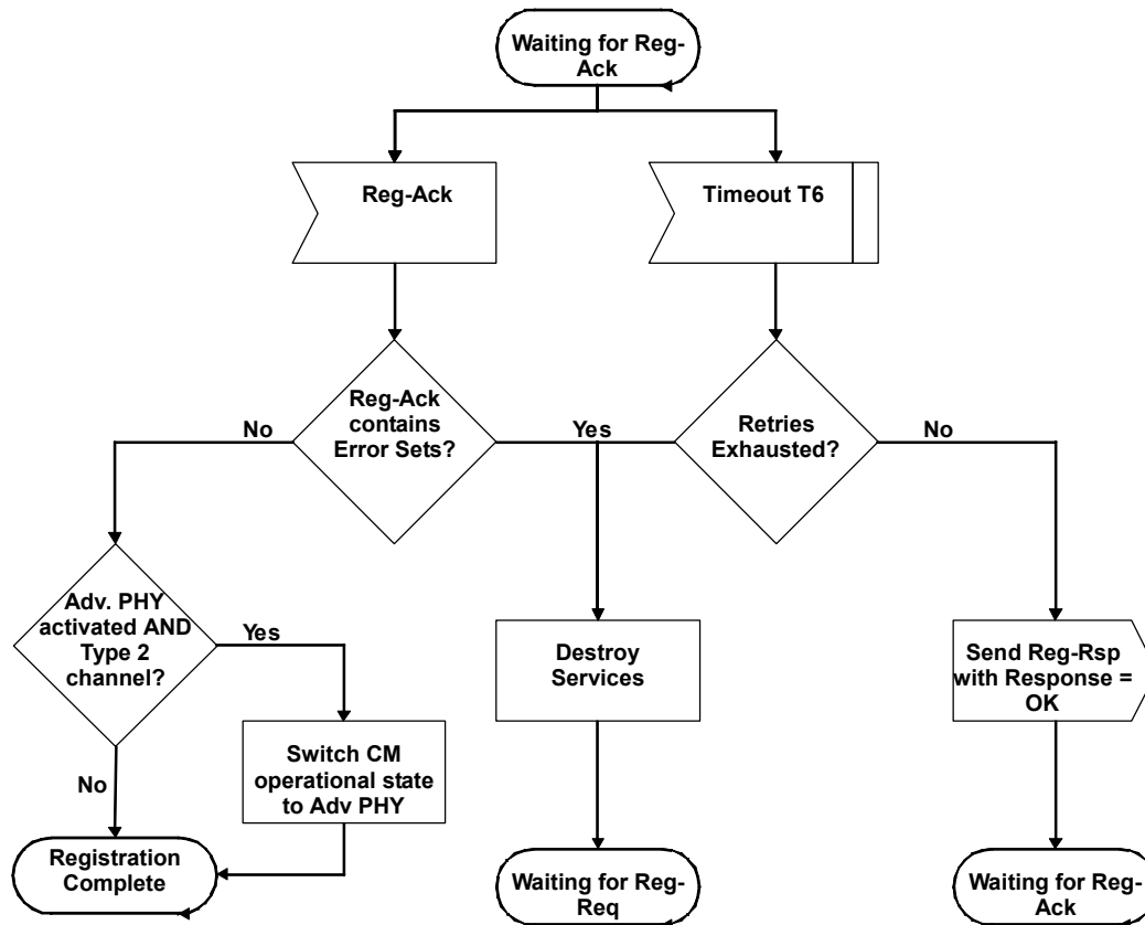
Figure 11–15 Registration Acknowledgment — CMTS
