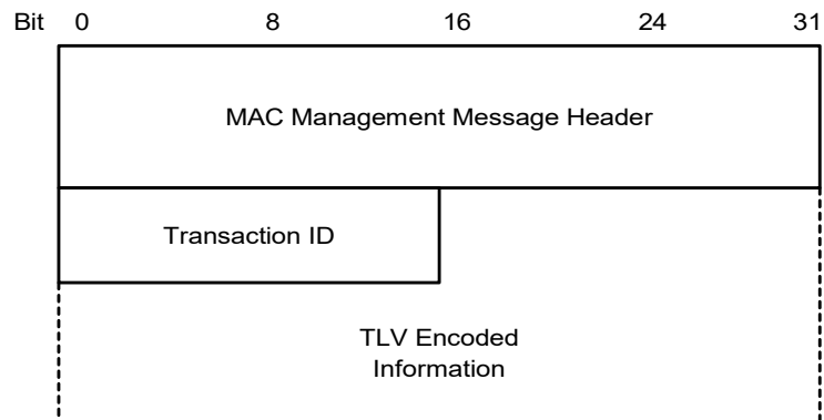
Figure 8–38 Dynamic Channel Change Request
