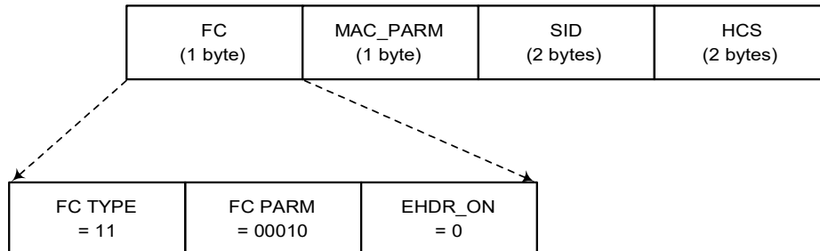
Figure 8–8 Request Frame Format
