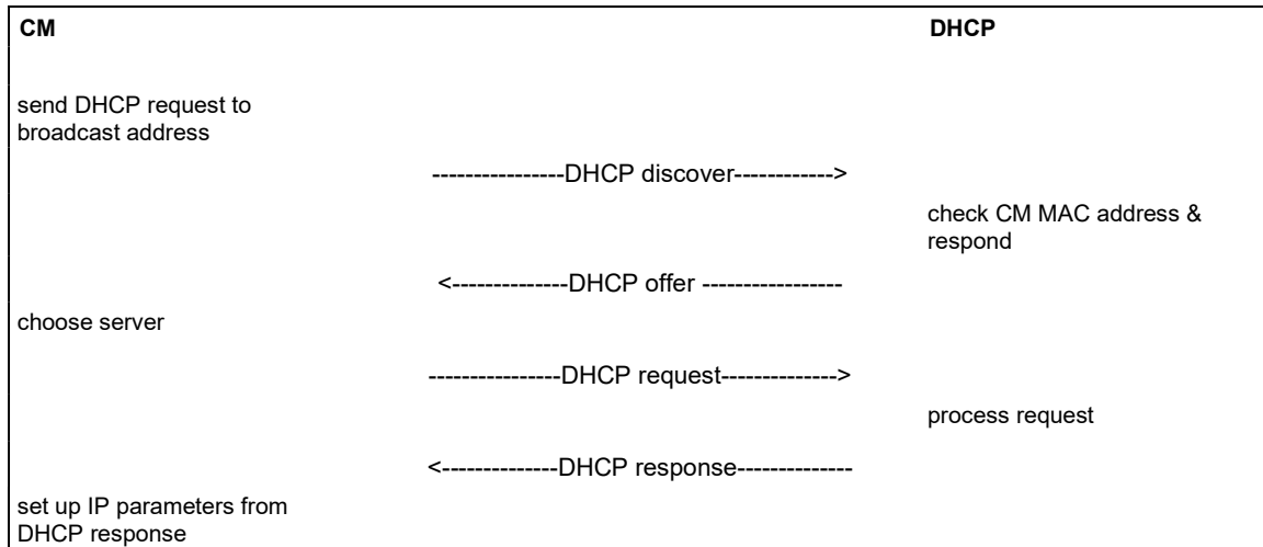
Figure 11–10 Establishing IP Connectivity
