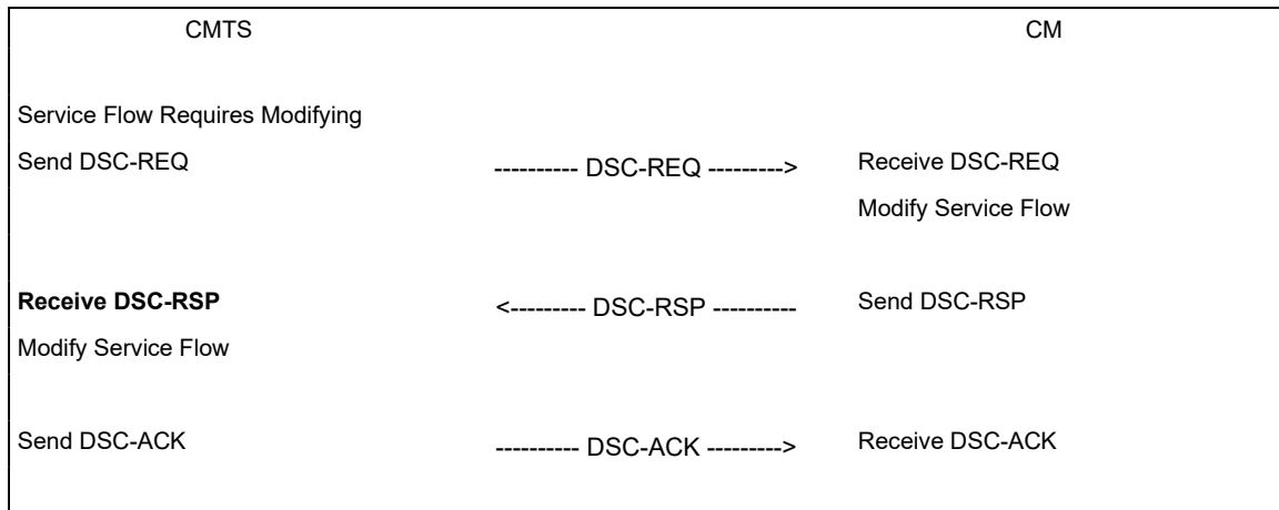
Figure 11–41 CMTS-Initiated DSC
