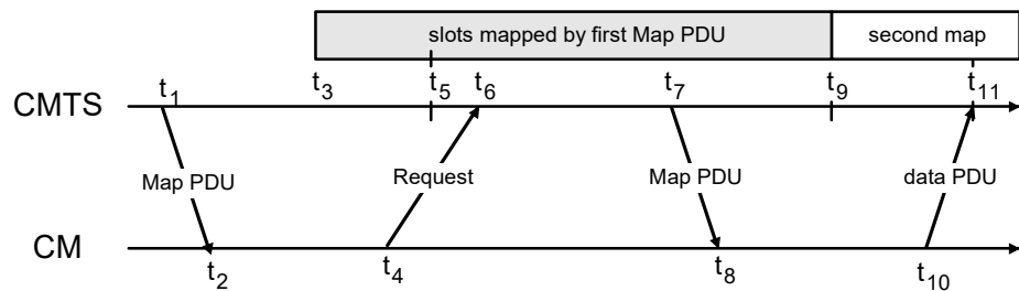
Figure 9–2 Protocol Example
