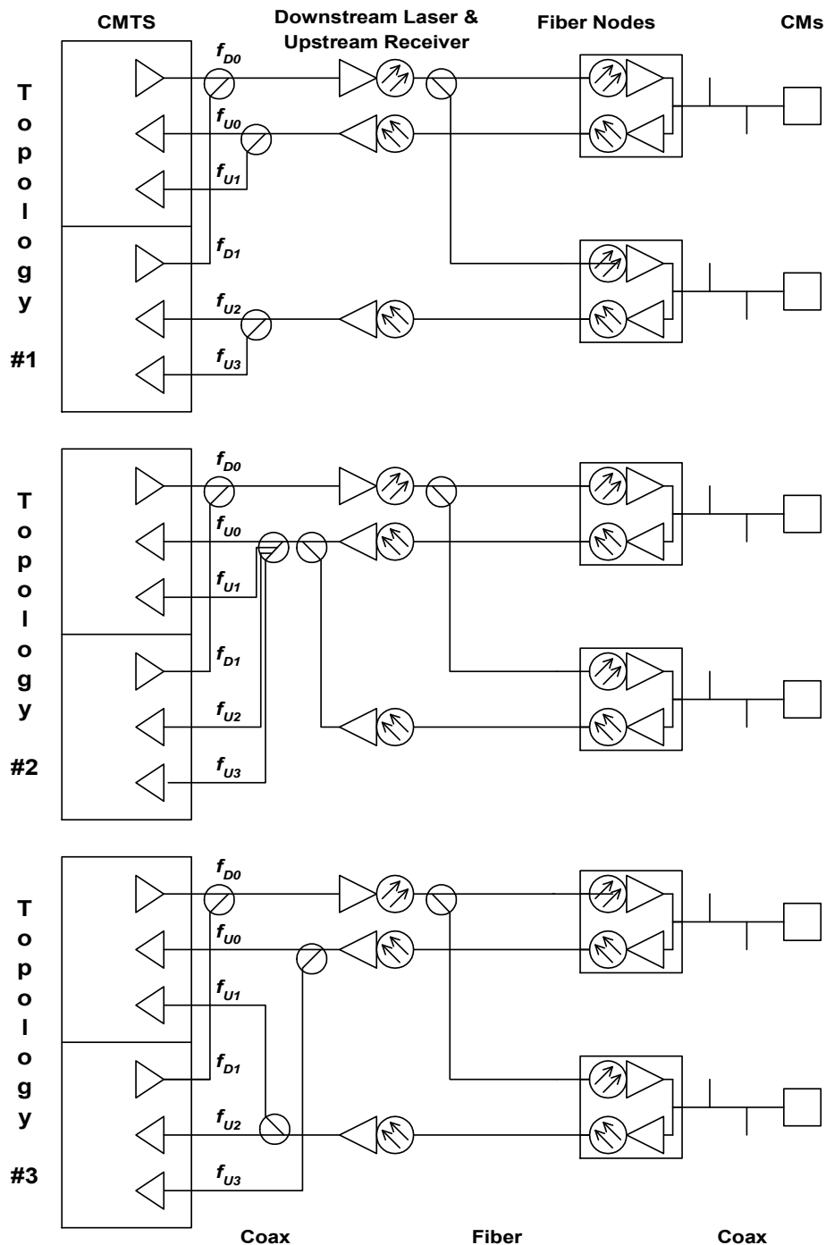
Figure III–2 Multiple Downstream and Multiple Upstream Channels per CM
