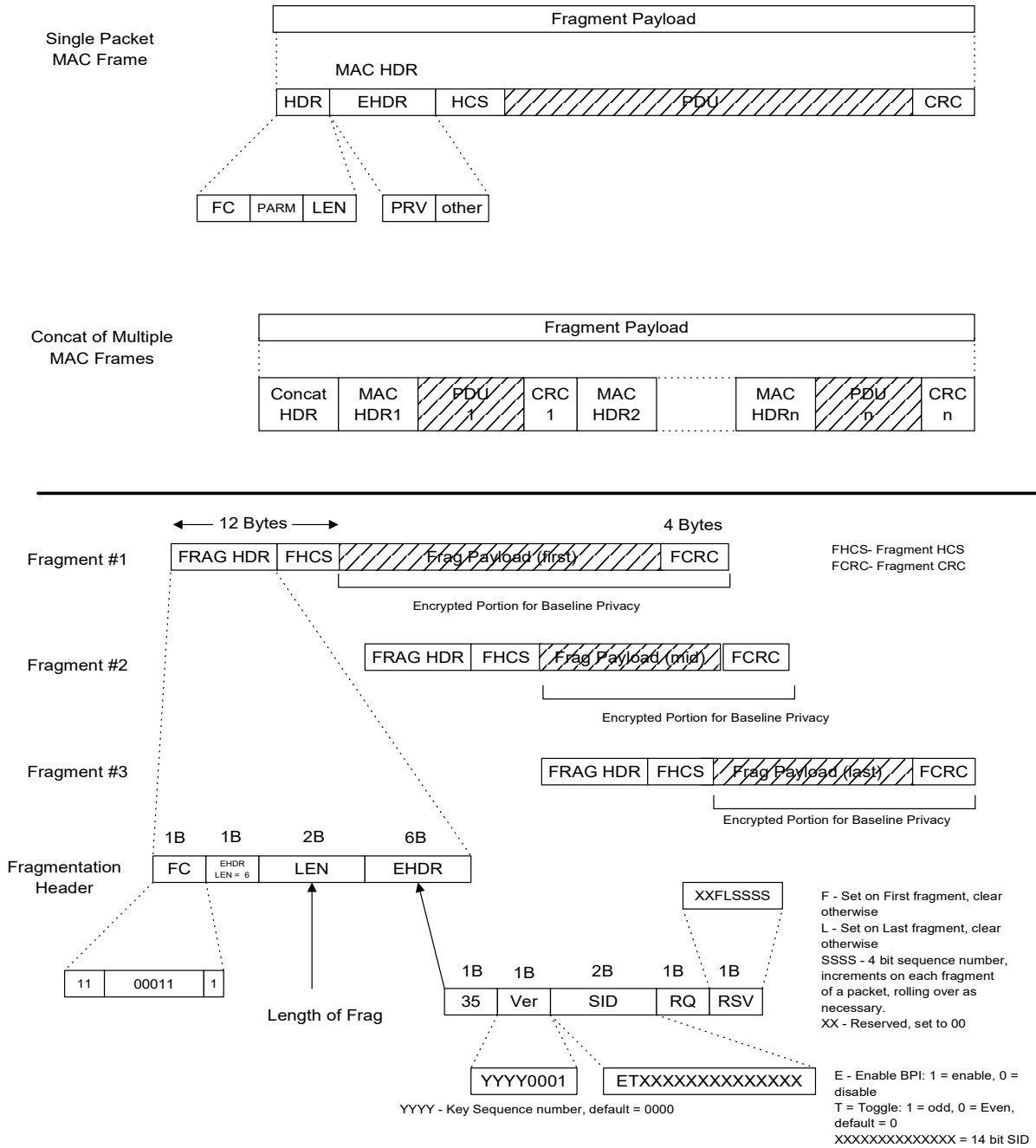
Figure 8–13 Fragmentation Details
