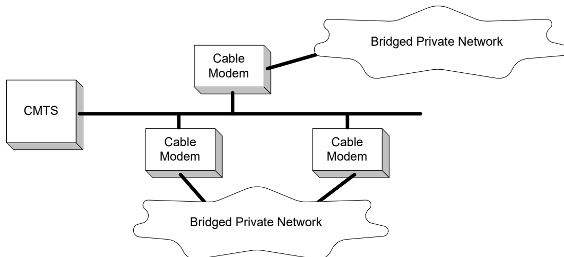
Figure E-1 Spanning Tree Topology
