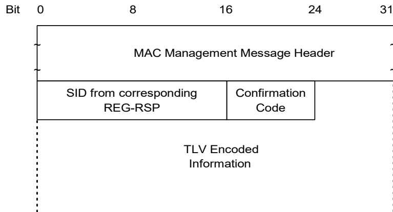
Figure 8–27 Registration Acknowledgment
